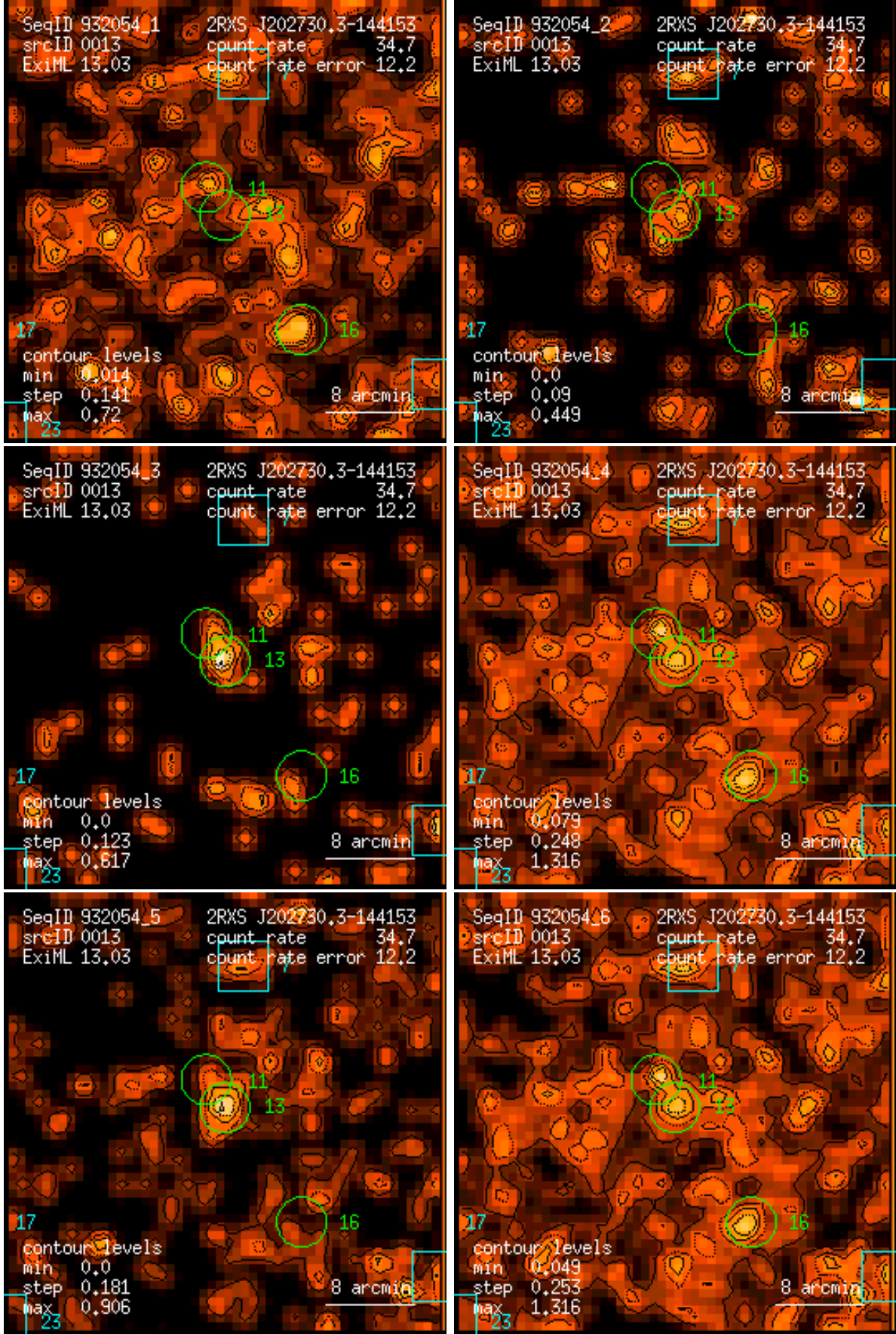
Figure 13: RASS 932054: detection 0013: band rate images, Gaussian filter: (1) PSPC channels 11 – 41, (2) 52 – 90, (3) 91 – 201, (4) 11 – 235, (5) 52 – 201, (6) 11 – 201. Broad band rates in counts/ks. Band rate contour levels in counts/ks/arcmin 2 .
