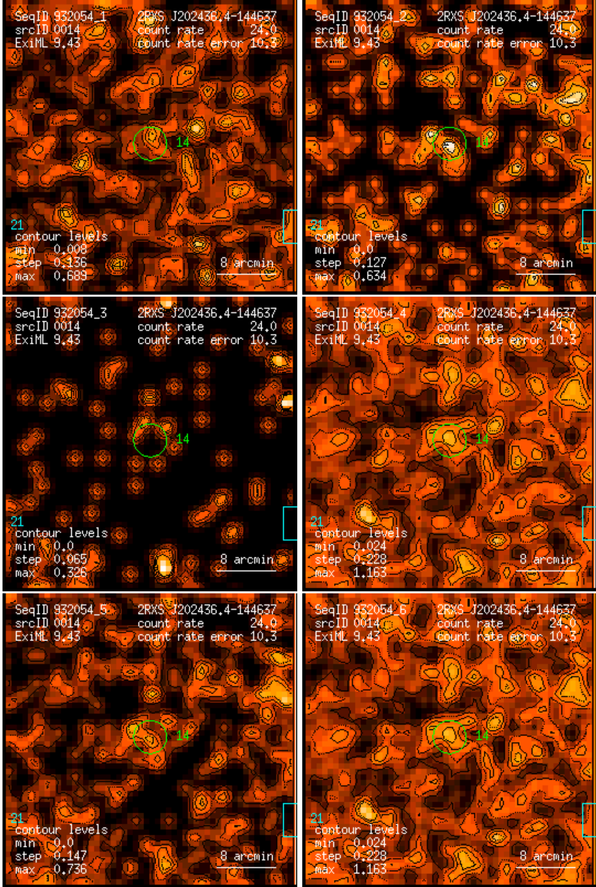
Figure 14: RASS 932054: detection 0014: band rate images, Gaussian filter: (1) PSPC channels 11 – 41, (2) 52 – 90, (3) 91 – 201, (4) 11 – 235, (5) 52 – 201, (6) 11 – 201. Broad band rates in counts/ks. Band rate contour levels in counts/ks/arcmin 2 .
