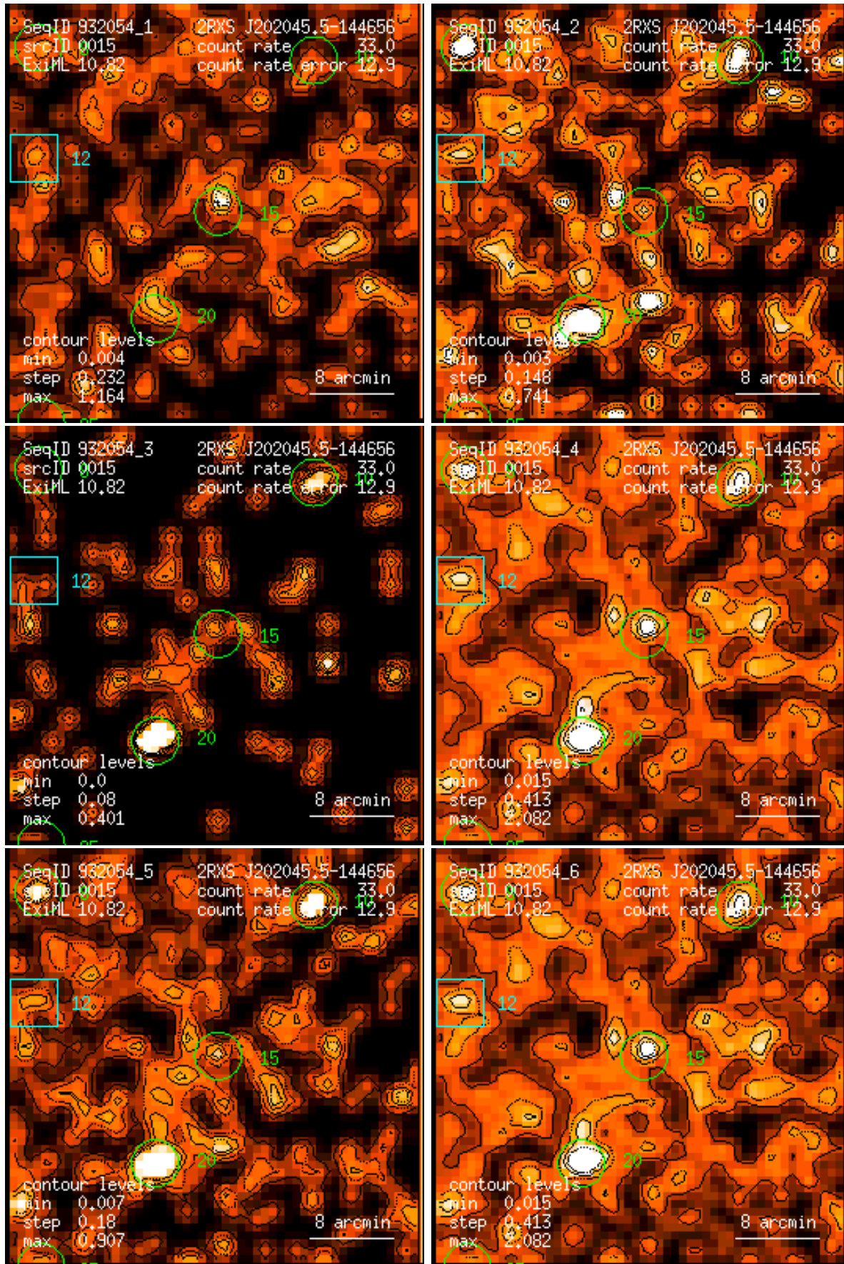
Figure 15: RASS 932054: detection 0015: band rate images, Gaussian filter: (1) PSPC channels 11 – 41, (2) 52 – 90, (3) 91 – 201, (4) 11 – 235, (5) 52 – 201, (6) 11 – 201. Broad band rates in counts/ks. Band rate contour levels in counts/ks/arcmin 2 .
