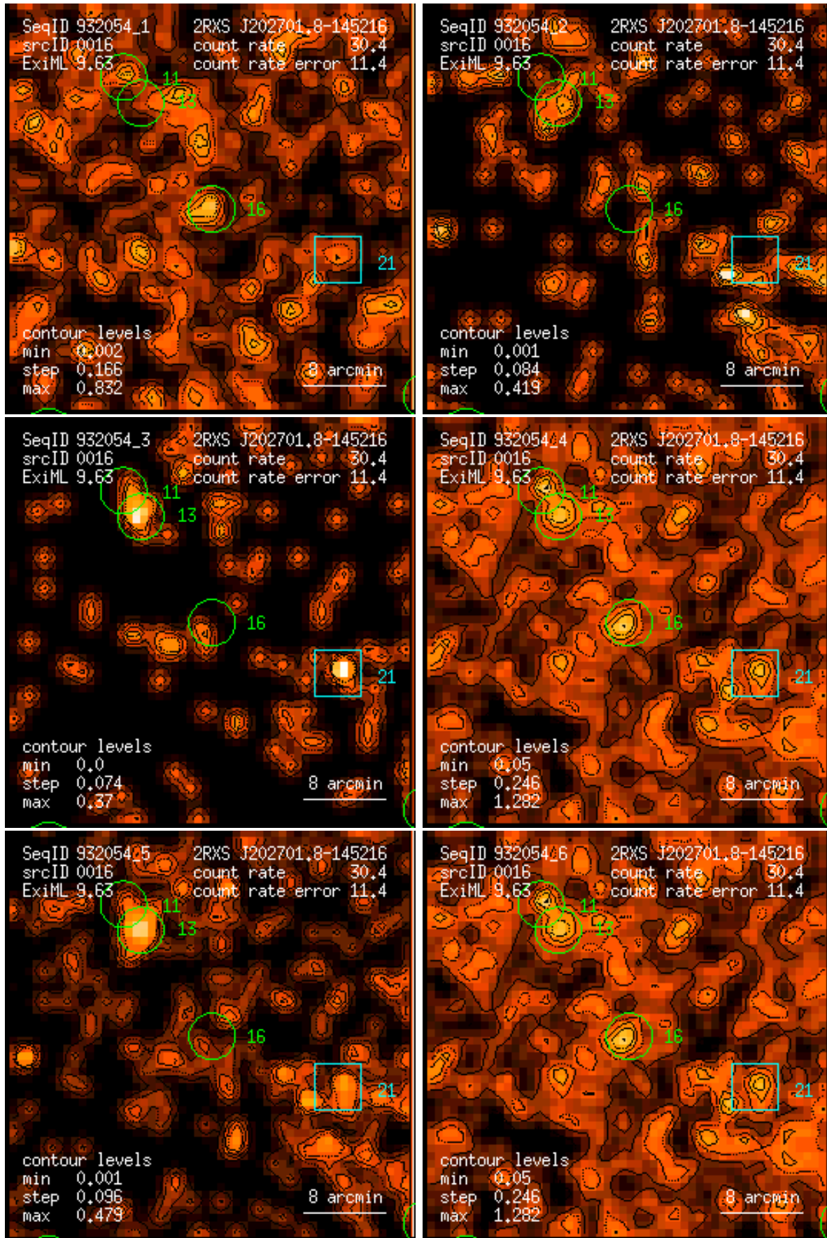
Figure 16: RASS 932054: detection 0016: band rate images, Gaussian filter: (1) PSPC channels 11 – 41, (2) 52 – 90, (3) 91 – 201, (4) 11 – 235, (5) 52 – 201, (6) 11 – 201. Broad band rates in counts/ks. Band rate contour levels in counts/ks/arcmin 2 .
