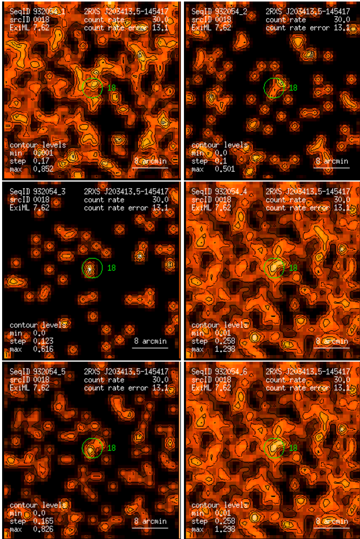
Figure 18: RASS 932054: detection 0018: band rate images, Gaussian filter: (1) PSPC channels 11 – 41, (2) 52 – 90, (3) 91 – 201, (4) 11 – 235, (5) 52 – 201, (6) 11 – 201. Broad band rates in counts/ks. Band rate contour levels in counts/ks/arcmin 2 .
