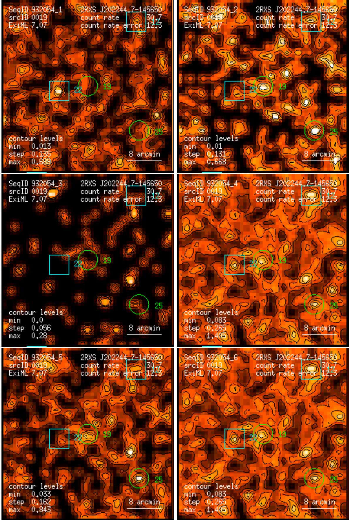
Figure 19: RASS 932054: detection 0019: band rate images, Gaussian filter: (1) PSPC channels 11 – 41, (2) 52 – 90, (3) 91 – 201, (4) 11 – 235, (5) 52 – 201, (6) 11 – 201. Broad band rates in counts/ks. Band rate contour levels in counts/ks/arcmin 2 .
