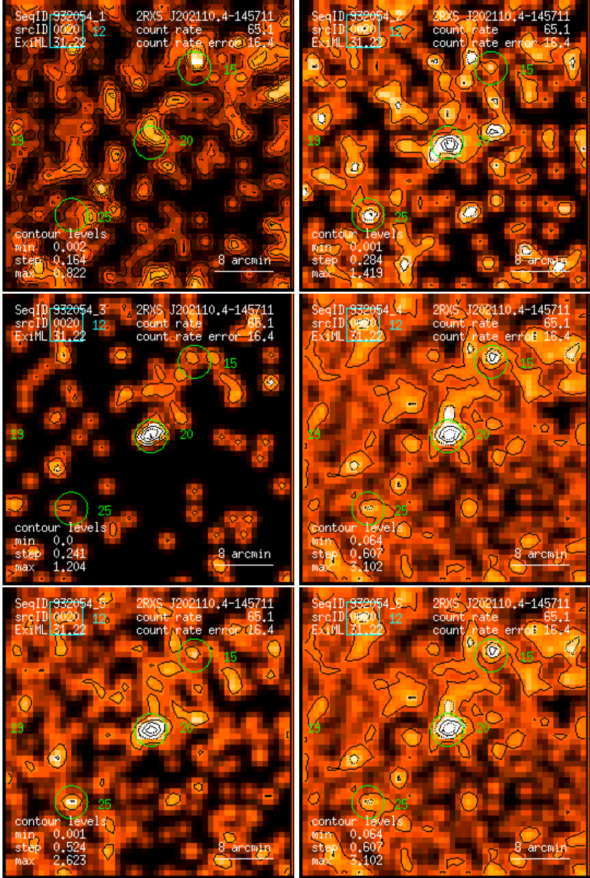
Figure 20: RASS 932054: detection 0020: band rate images, Gaussian filter: (1) PSPC channels 11 – 41, (2) 52 – 90, (3) 91 – 201, (4) 11 – 235, (5) 52 – 201, (6) 11 – 201. Broad band rates in counts/ks. Band rate contour levels in counts/ks/arcmin 2 .
