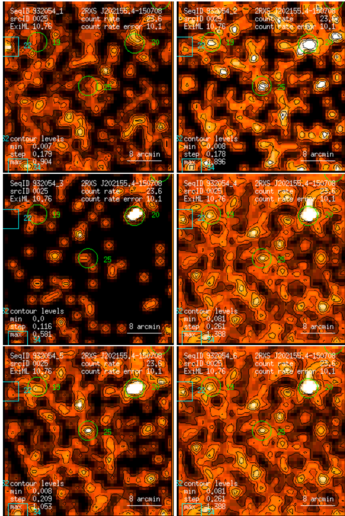
Figure 25: RASS 932054: detection 0025: band rate images, Gaussian filter: (1) PSPC channels 11 – 41, (2) 52 – 90, (3) 91 – 201, (4) 11 – 235, (5) 52 – 201, (6) 11 – 201. Broad band rates in counts/ks. Band rate contour levels in counts/ks/arcmin 2 .
