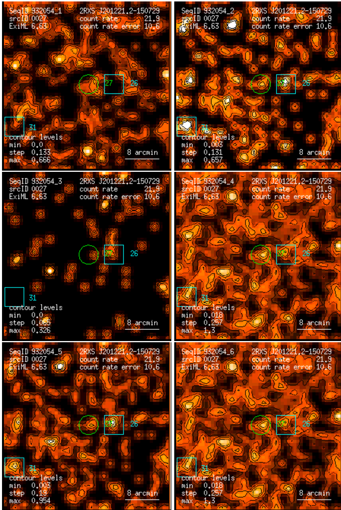
Figure 27: RASS 932054: detection 0027: band rate images, Gaussian filter: (1) PSPC channels 11 – 41, (2) 52 – 90, (3) 91 – 201, (4) 11 – 235, (5) 52 – 201, (6) 11 – 201. Broad band rates in counts/ks. Band rate contour levels in counts/ks/arcmin 2 .
