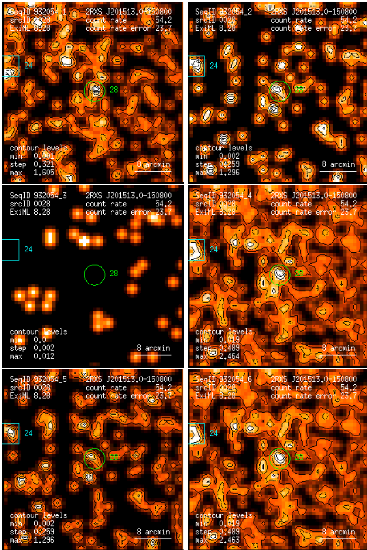
Figure 28: RASS 932054: detection 0028: band rate images, Gaussian filter: (1) PSPC channels 11 – 41, (2) 52 – 90, (3) 91 – 201, (4) 11 – 235, (5) 52 – 201, (6) 11 – 201. Broad band rates in counts/ks. Band rate contour levels in counts/ks/arcmin 2 .
