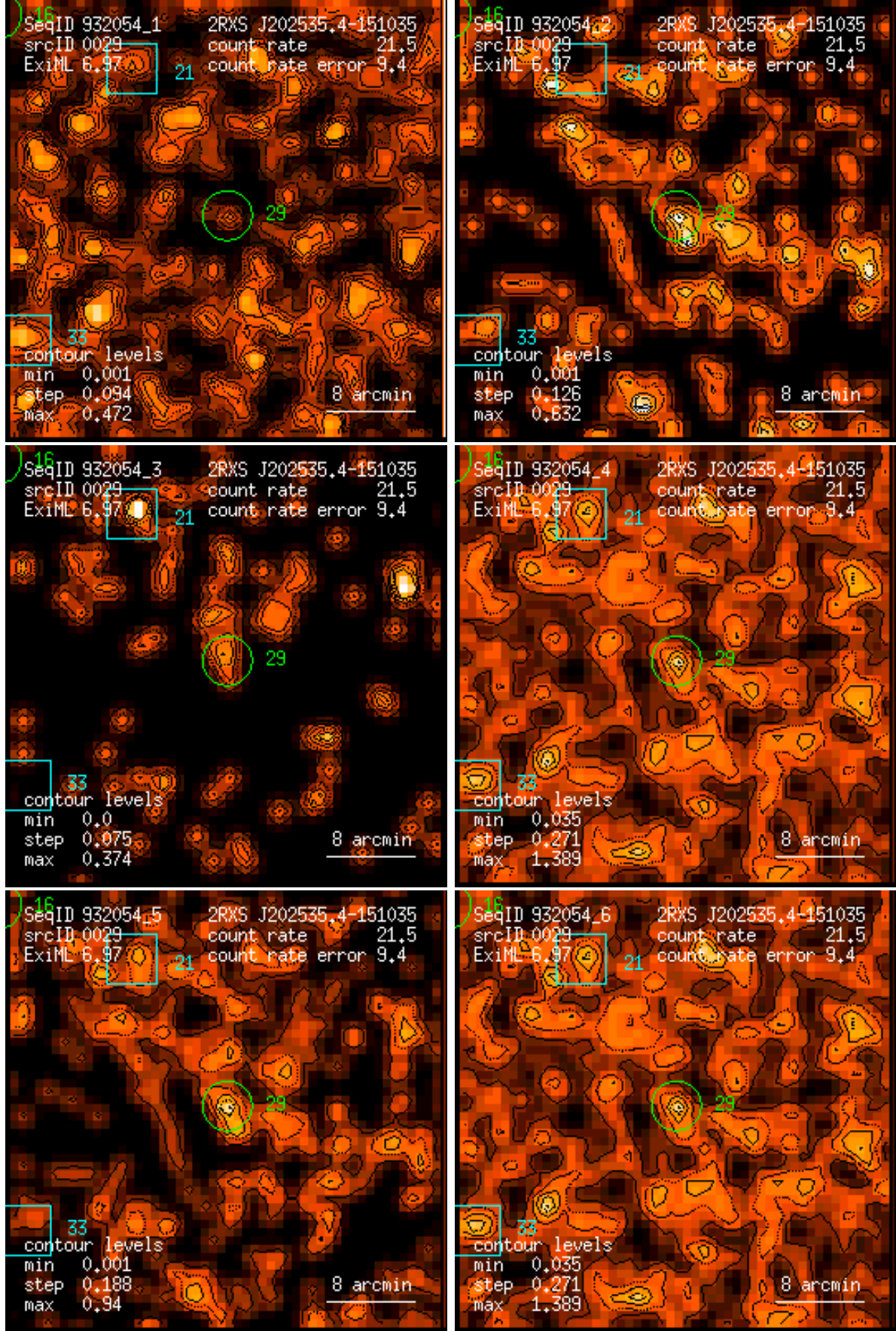
Figure 29: RASS 932054: detection 0029: band rate images, Gaussian filter: (1) PSPC channels 11 – 41, (2) 52 – 90, (3) 91 – 201, (4) 11 – 235, (5) 52 – 201, (6) 11 – 201. Broad band rates in counts/ks. Band rate contour levels in counts/ks/arcmin 2 .
