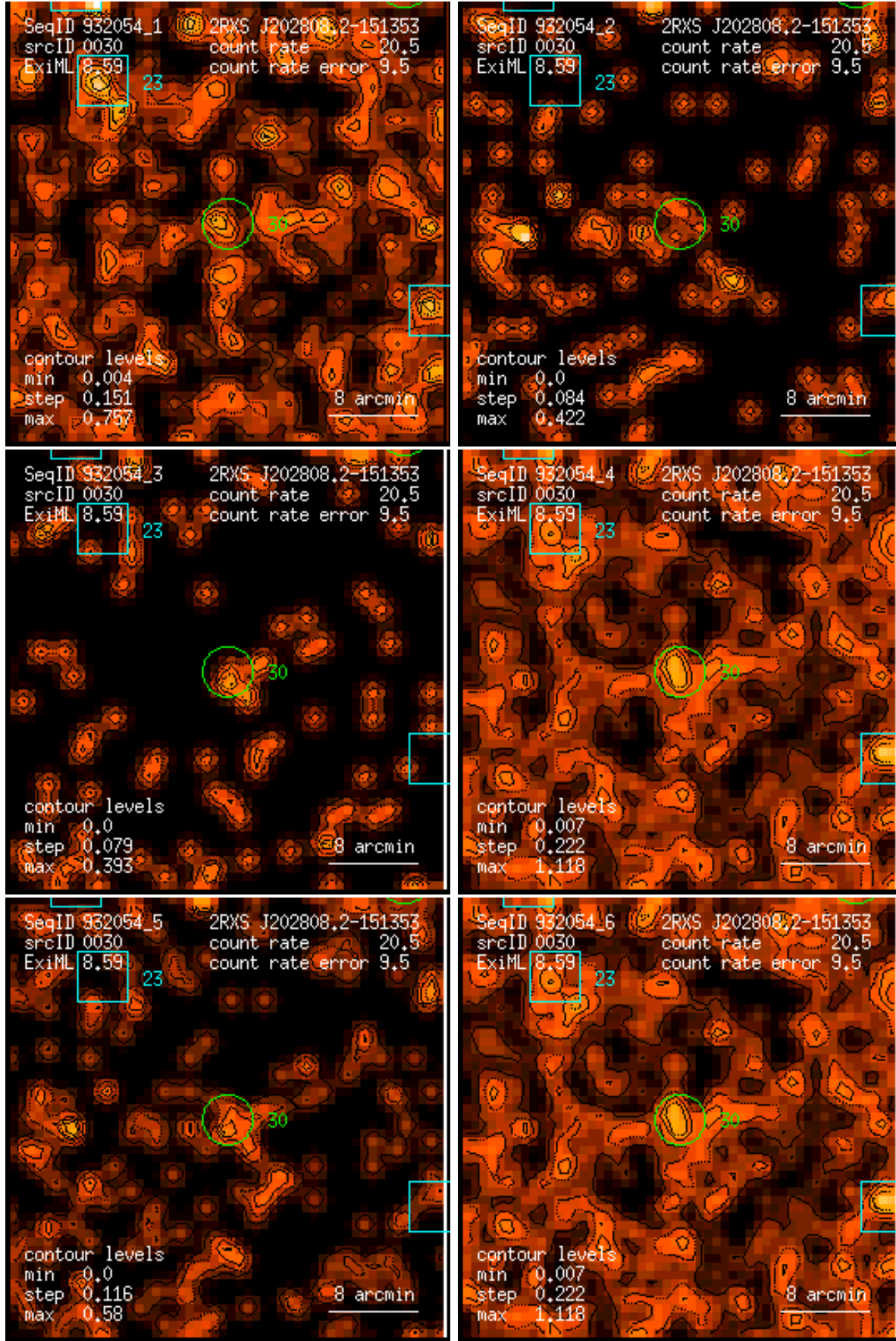
Figure 30: RASS 932054: detection 0030: band rate images, Gaussian filter: (1) PSPC channels 11 – 41, (2) 52 – 90, (3) 91 – 201, (4) 11 – 235, (5) 52 – 201, (6) 11 – 201. Broad band rates in counts/ks. Band rate contour levels in counts/ks/arcmin 2 .
