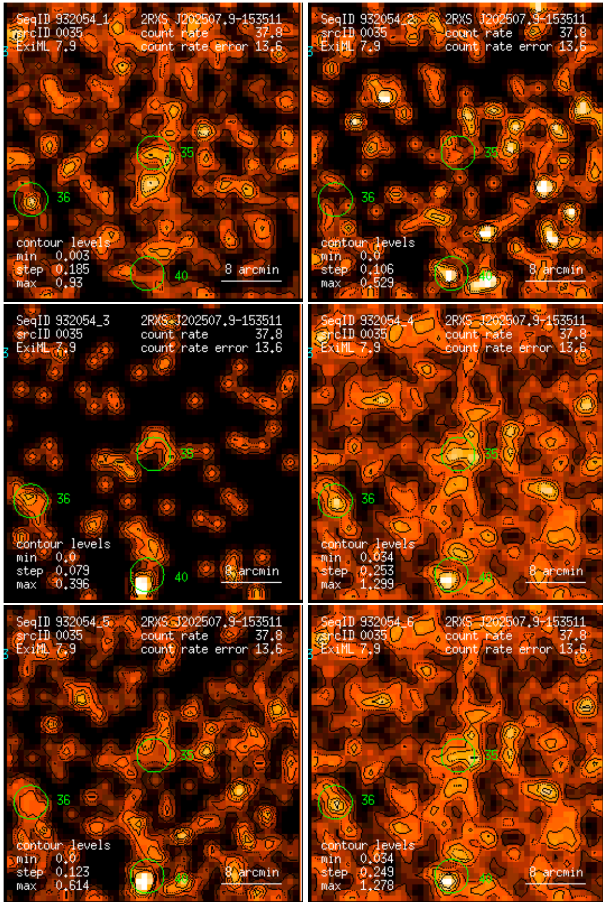
Figure 35: RASS 932054: detection 0035: band rate images, Gaussian filter: (1) PSPC channels 11 – 41, (2) 52 – 90, (3) 91 – 201, (4) 11 – 235, (5) 52 – 201, (6) 11 – 201. Broad band rates in counts/ks. Band rate contour levels in counts/ks/arcmin 2 .
