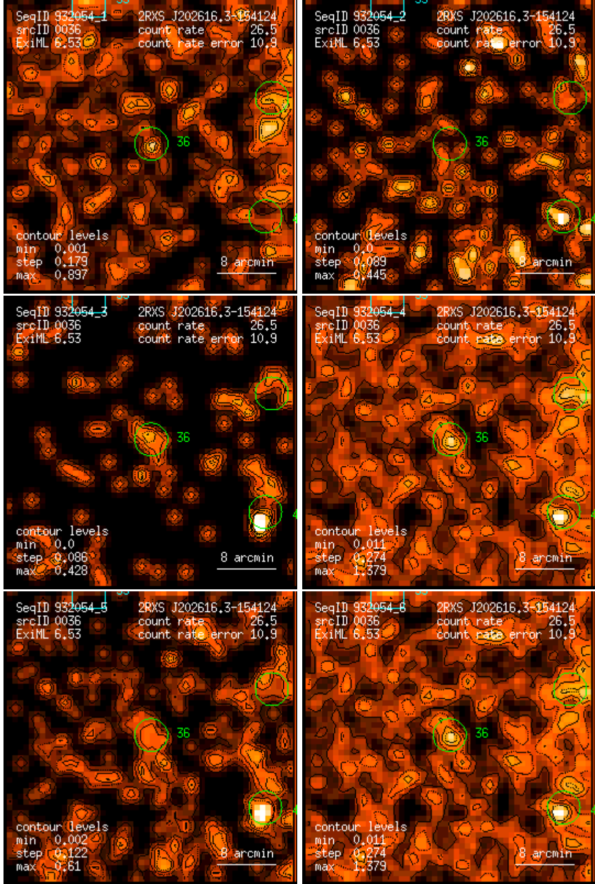
Figure 36: RASS 932054: detection 0036: band rate images, Gaussian filter: (1) PSPC channels 11 – 41, (2) 52 – 90, (3) 91 – 201, (4) 11 – 235, (5) 52 – 201, (6) 11 – 201. Broad band rates in counts/ks. Band rate contour levels in counts/ks/arcmin 2 .
