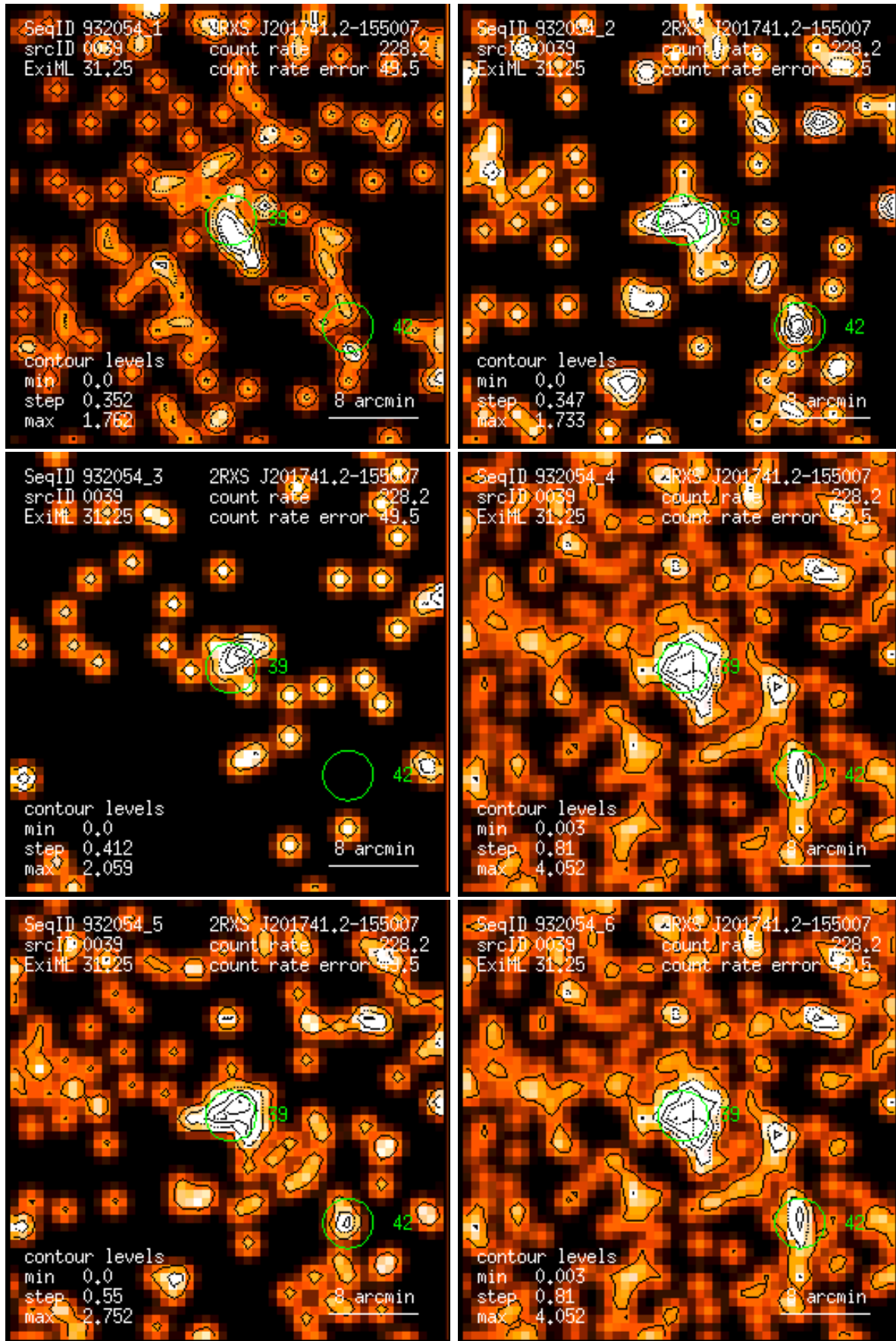
Figure 39: RASS 932054: detection 0039: band rate images, Gaussian filter: (1) PSPC channels 11 – 41, (2) 52 – 90, (3) 91 – 201, (4) 11 – 235, (5) 52 – 201, (6) 11 – 201. Broad band rates in counts/ks. Band rate contour levels in counts/ks/arcmin 2 .
