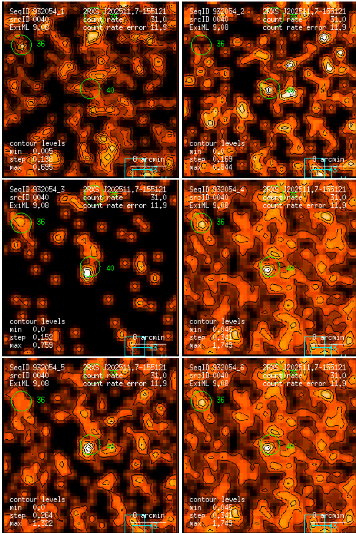
Figure 40: RASS 932054: detection 0040: band rate images, Gaussian filter: (1) PSPC channels 11 – 41, (2) 52 – 90, (3) 91 – 201, (4) 11 – 235, (5) 52 – 201, (6) 11 – 201. Broad band rates in counts/ks. Band rate contour levels in counts/ks/arcmin 2 .
