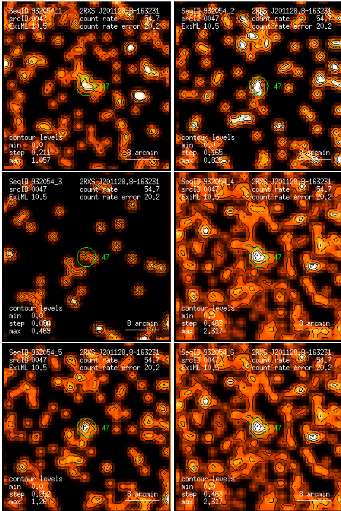
Figure 47: RASS 932054: detection 0047: band rate images, Gaussian filter: (1) PSPC channels 11 – 41, (2) 52 – 90, (3) 91 – 201, (4) 11 – 235, (5) 52 – 201, (6) 11 – 201. Broad band rates in counts/ks. Band rate contour levels in counts/ks/arcmin 2 .
