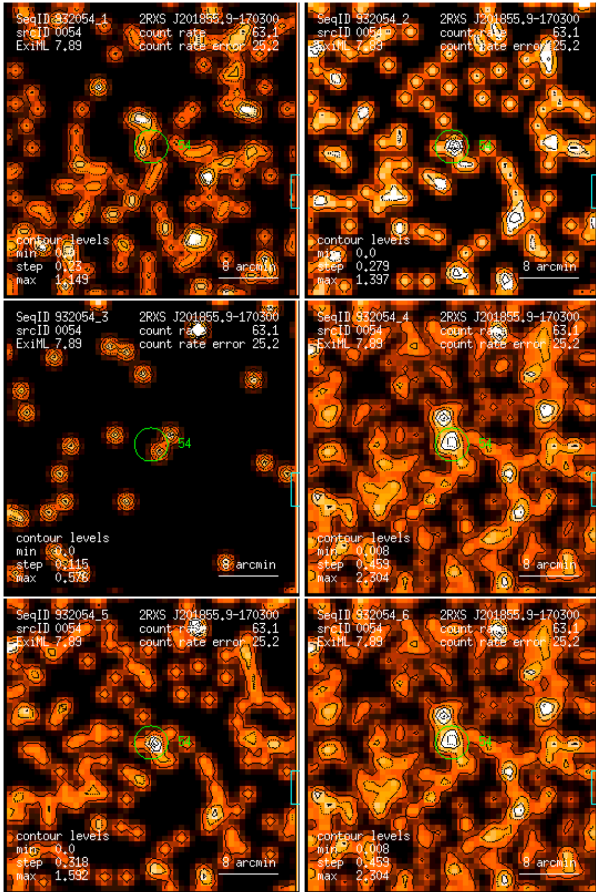
Figure 54: RASS 932054: detection 0054: band rate images, Gaussian filter: (1) PSPC channels 11 – 41, (2) 52 – 90, (3) 91 – 201, (4) 11 – 235, (5) 52 – 201, (6) 11 – 201. Broad band rates in counts/ks. Band rate contour levels in counts/ks/arcmin 2 .
