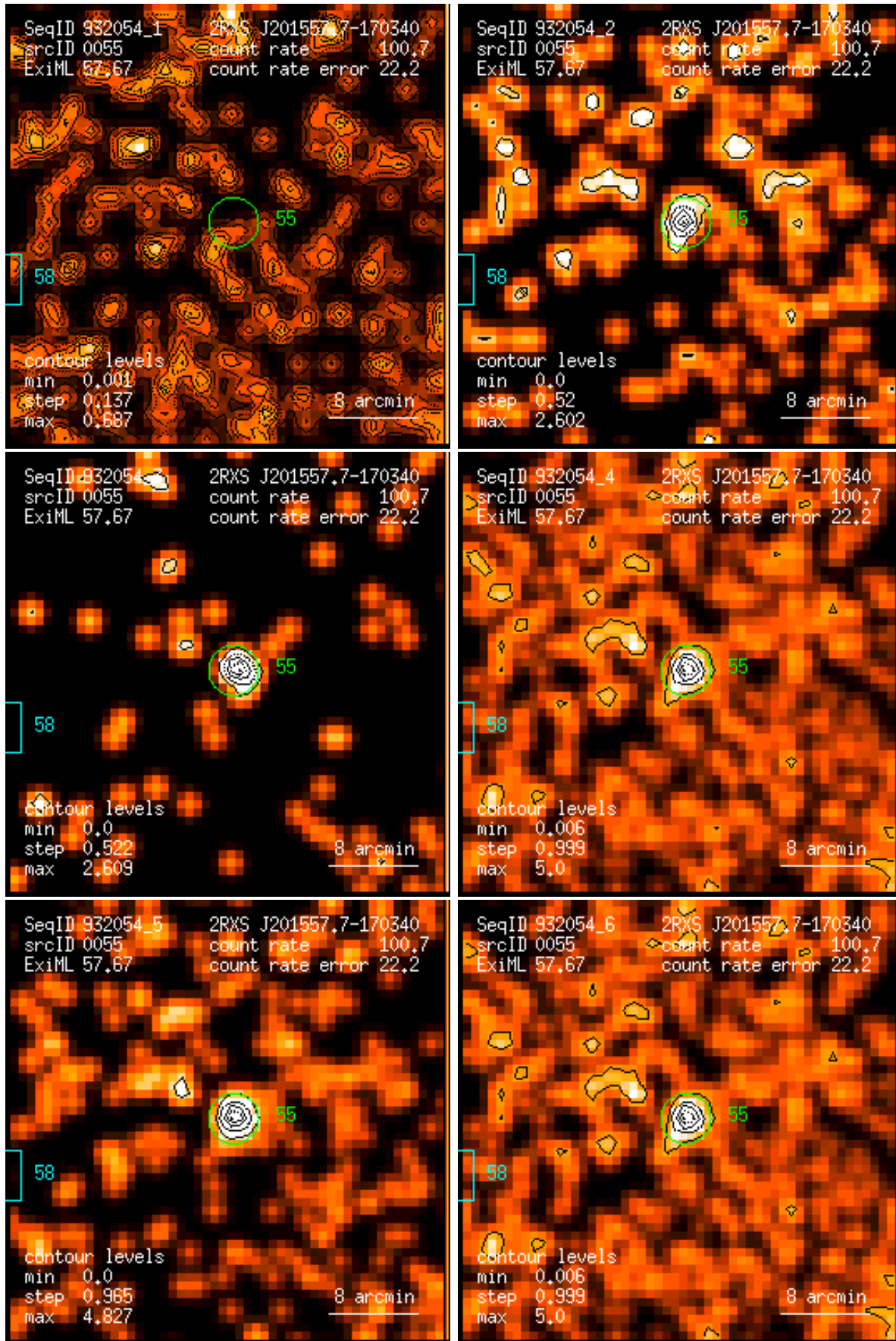
Figure 55: RASS 932054: detection 0055: band rate images, Gaussian filter: (1) PSPC channels 11 – 41, (2) 52 – 90, (3) 91 – 201, (4) 11 – 235, (5) 52 – 201, (6) 11 – 201. Broad band rates in counts/ks. Band rate contour levels in counts/ks/arcmin 2 .
