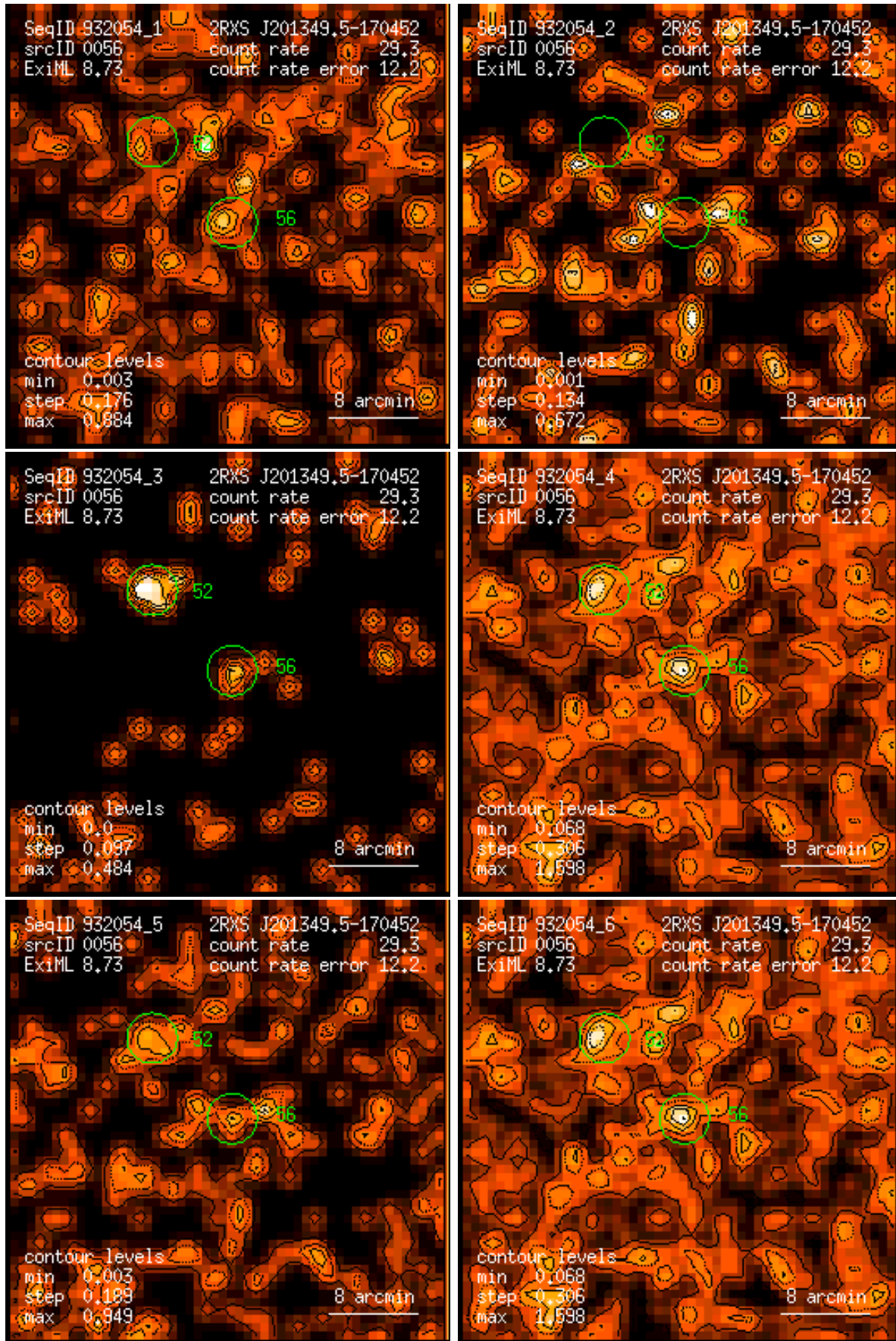
Figure 56: RASS 932054: detection 0056: band rate images, Gaussian filter: (1) PSPC channels 11 – 41, (2) 52 – 90, (3) 91 – 201, (4) 11 – 235, (5) 52 – 201, (6) 11 – 201. Broad band rates in counts/ks. Band rate contour levels in counts/ks/arcmin 2 .
