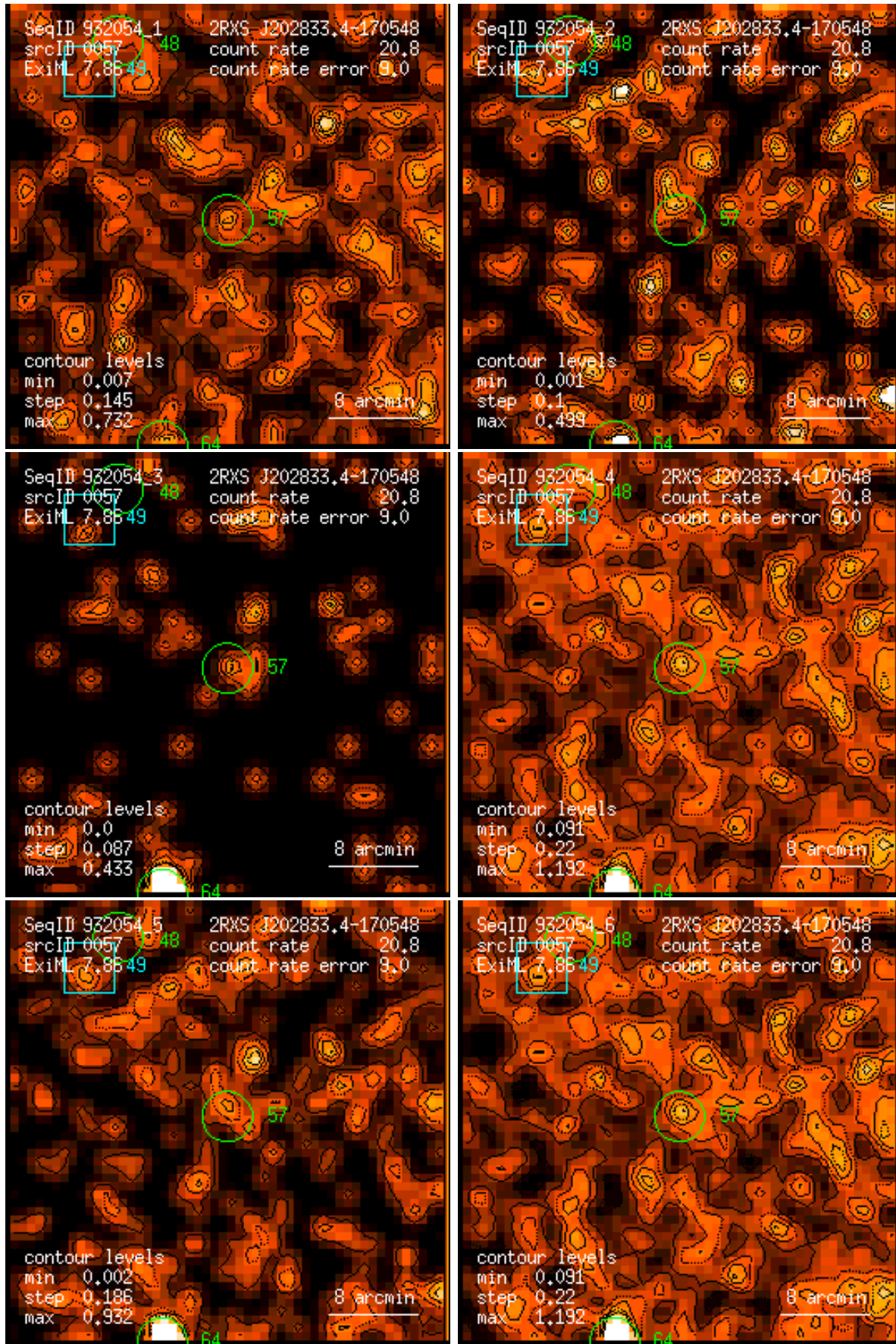
Figure 57: RASS 932054: detection 0057: band rate images, Gaussian filter: (1) PSPC channels 11 – 41, (2) 52 – 90, (3) 91 – 201, (4) 11 – 235, (5) 52 – 201, (6) 11 – 201. Broad band rates in counts/ks. Band rate contour levels in counts/ks/arcmin 2 .
