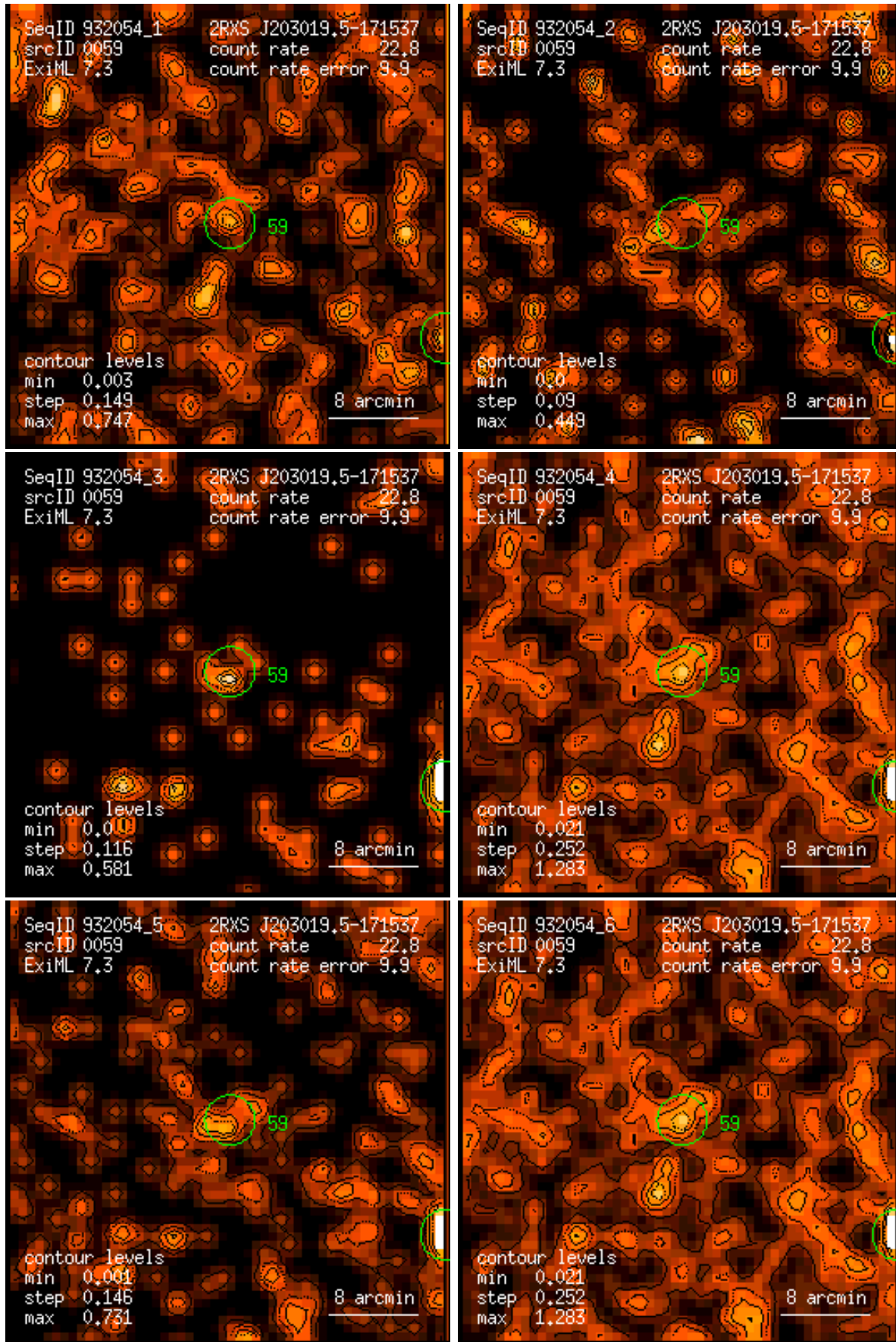
Figure 59: RASS 932054: detection 0059: band rate images, Gaussian filter: (1) PSPC channels 11 – 41, (2) 52 – 90, (3) 91 – 201, (4) 11 – 235, (5) 52 – 201, (6) 11 – 201. Broad band rates in counts/ks. Band rate contour levels in counts/ks/arcmin 2 .
