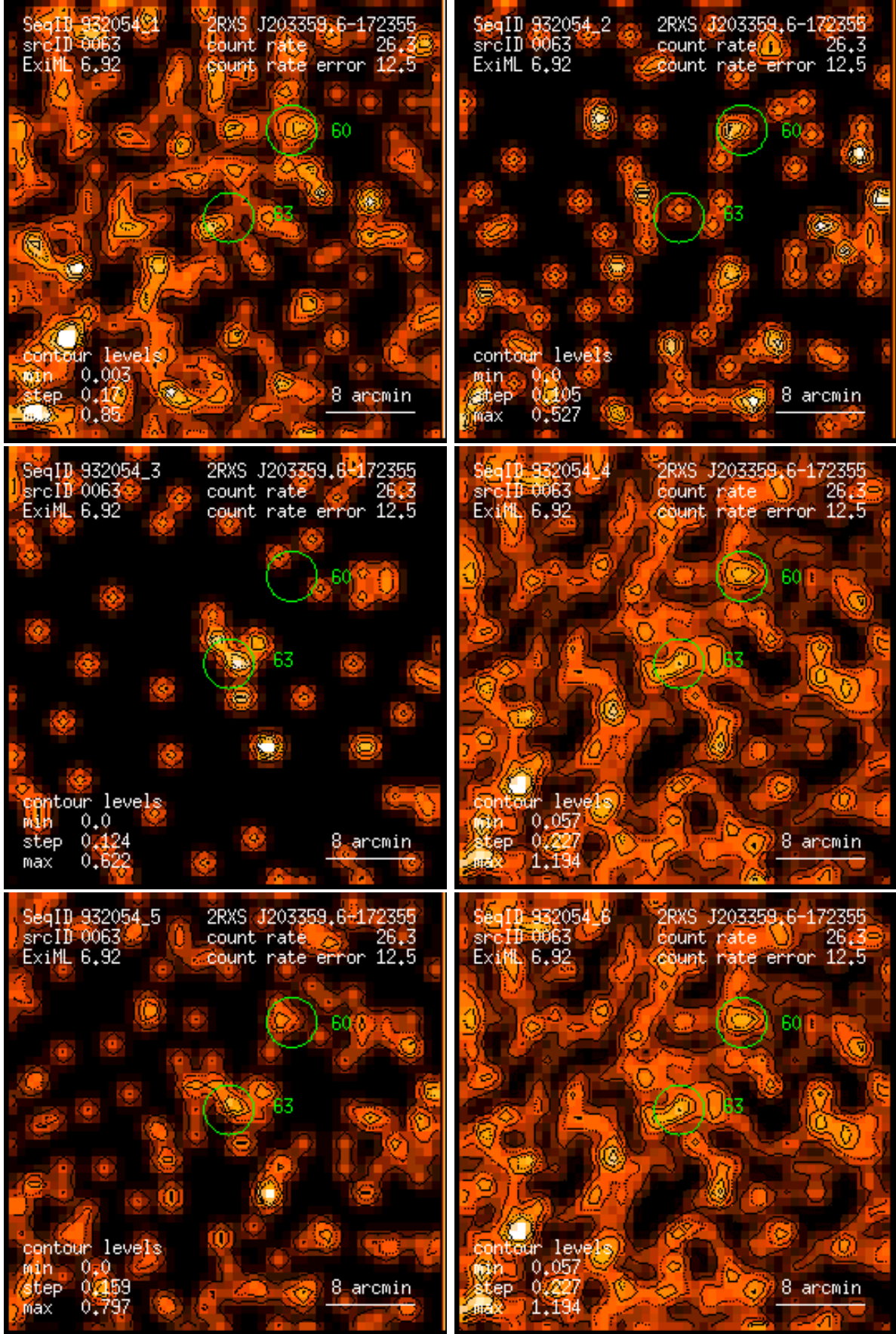
Figure 63: RASS 932054: detection 0063: band rate images, Gaussian filter: (1) PSPC channels 11 – 41, (2) 52 – 90, (3) 91 – 201, (4) 11 – 235, (5) 52 – 201, (6) 11 – 201. Broad band rates in counts/ks. Band rate contour levels in counts/ks/arcmin 2 .
