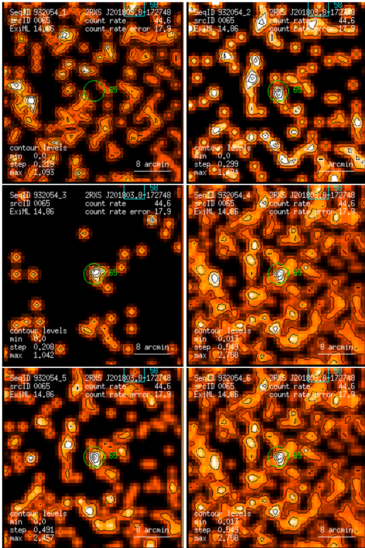
Figure 65: RASS 932054: detection 0065: band rate images, Gaussian filter: (1) PSPC channels 11 – 41, (2) 52 – 90, (3) 91 – 201, (4) 11 – 235, (5) 52 – 201, (6) 11 – 201. Broad band rates in counts/ks. Band rate contour levels in counts/ks/arcmin 2 .
