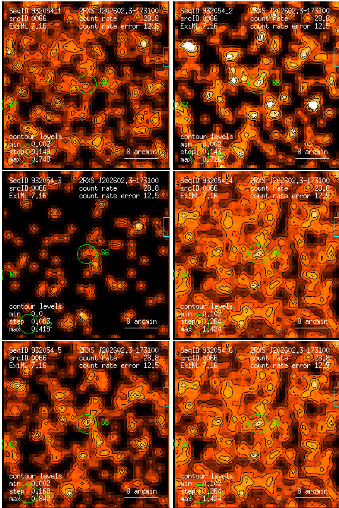
Figure 66: RASS 932054: detection 0066: band rate images, Gaussian filter: (1) PSPC channels 11 – 41, (2) 52 – 90, (3) 91 – 201, (4) 11 – 235, (5) 52 – 201, (6) 11 – 201. Broad band rates in counts/ks. Band rate contour levels in counts/ks/arcmin 2 .
