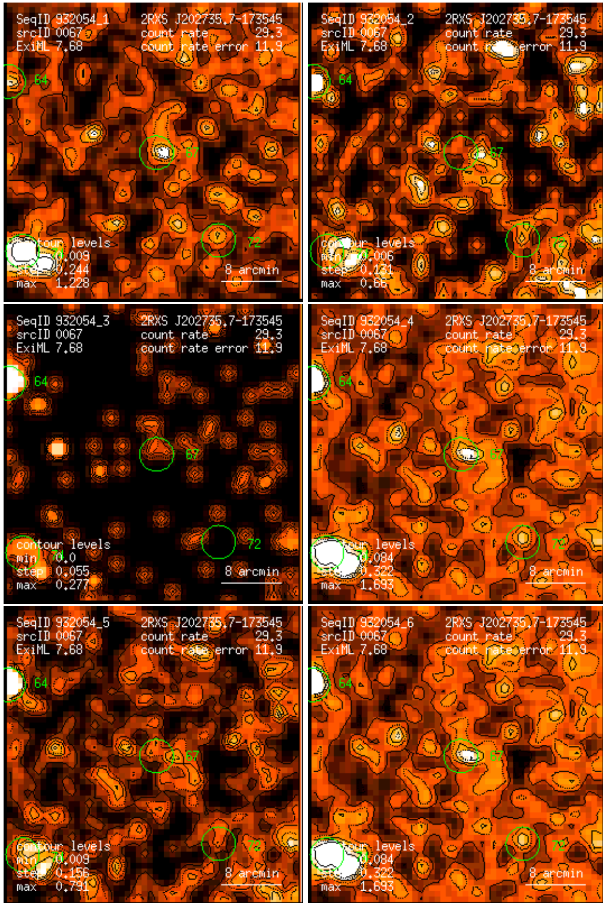
Figure 67: RASS 932054: detection 0067: band rate images, Gaussian filter: (1) PSPC channels 11 – 41, (2) 52 – 90, (3) 91 – 201, (4) 11 – 235, (5) 52 – 201, (6) 11 – 201. Broad band rates in counts/ks. Band rate contour levels in counts/ks/arcmin 2 .
