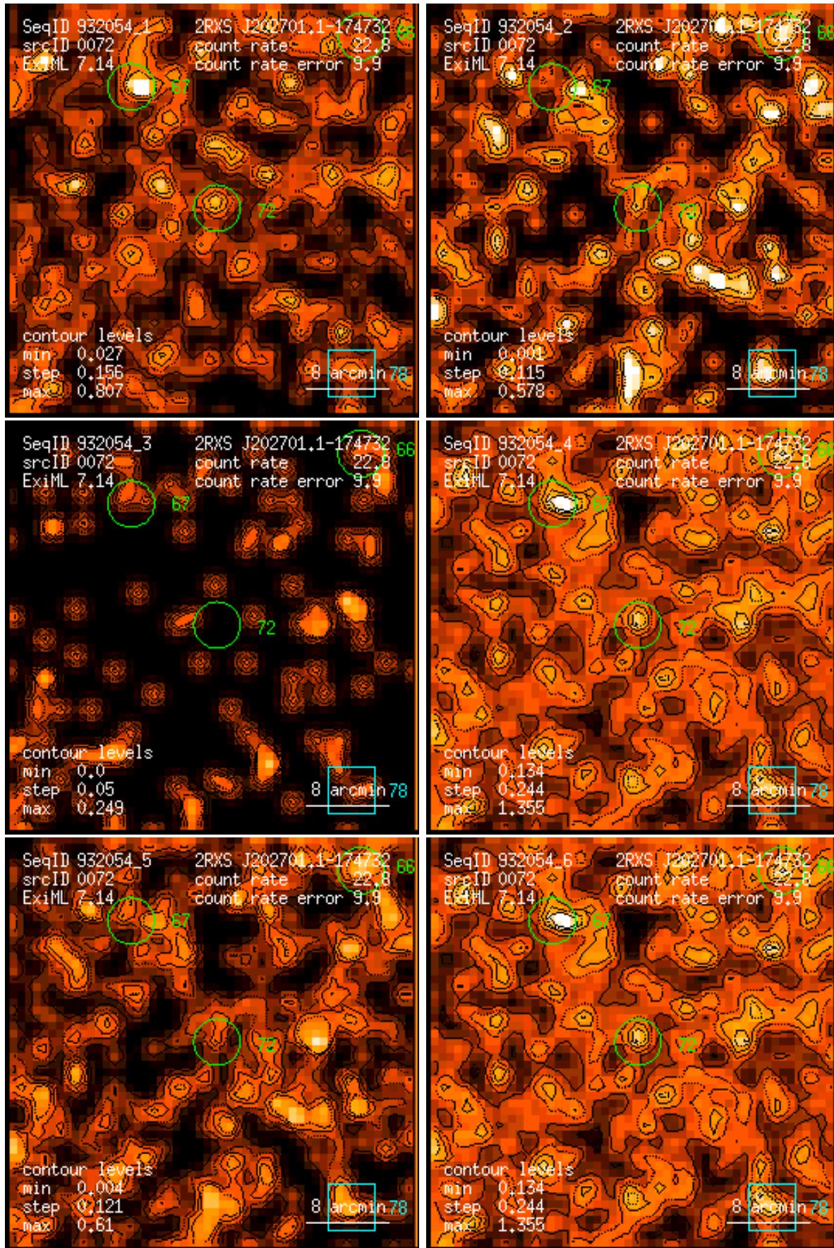
Figure 72: RASS 932054: detection 0072: band rate images, Gaussian filter: (1) PSPC channels 11 – 41, (2) 52 – 90, (3) 91 – 201, (4) 11 – 235, (5) 52 – 201, (6) 11 – 201. Broad band rates in counts/ks. Band rate contour levels in counts/ks/arcmin 2 .
