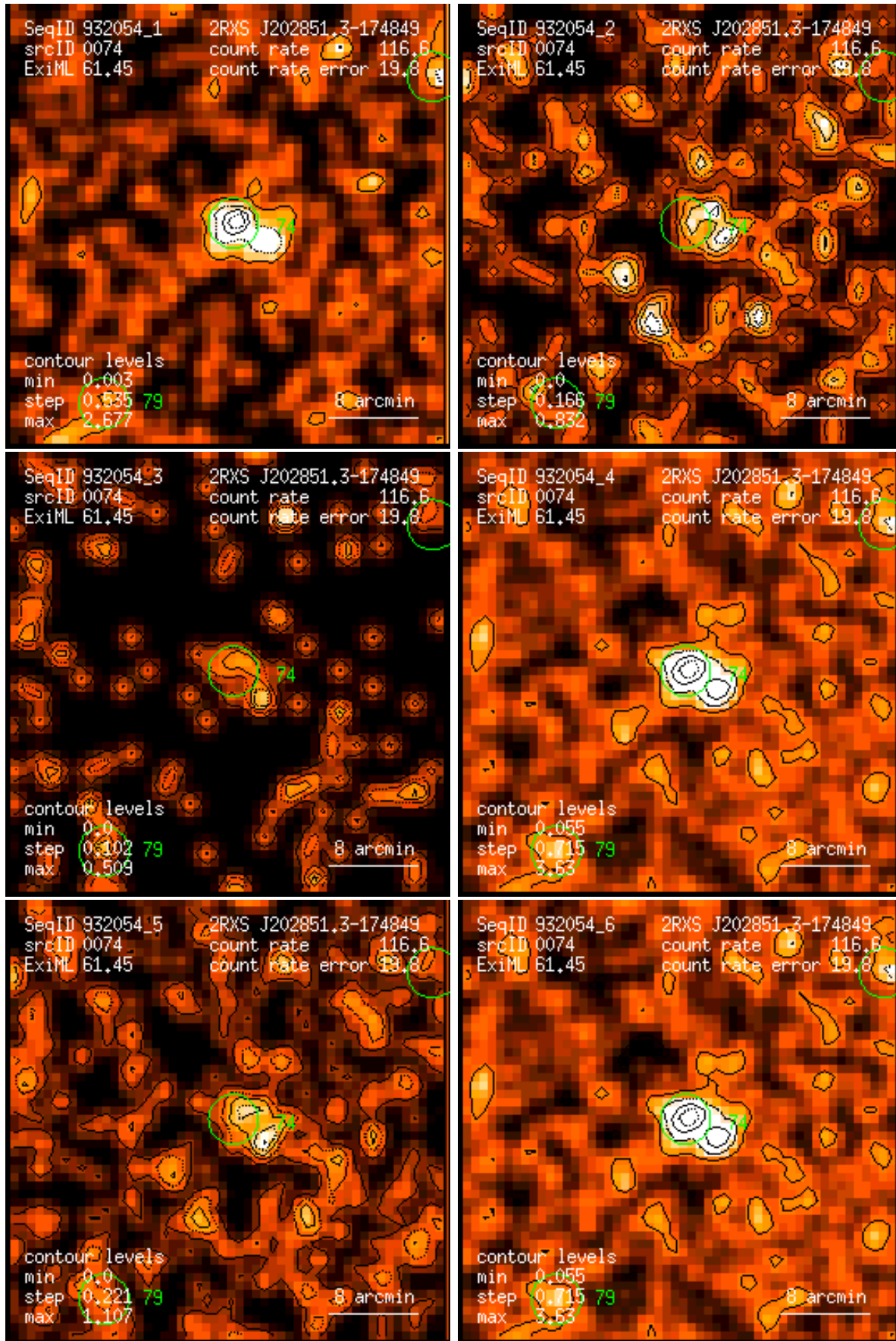
Figure 74: RASS 932054: detection 0074: band rate images, Gaussian filter: (1) PSPC channels 11 – 41, (2) 52 – 90, (3) 91 – 201, (4) 11 – 235, (5) 52 – 201, (6) 11 – 201. Broad band rates in counts/ks. Band rate contour levels in counts/ks/arcmin 2 .
