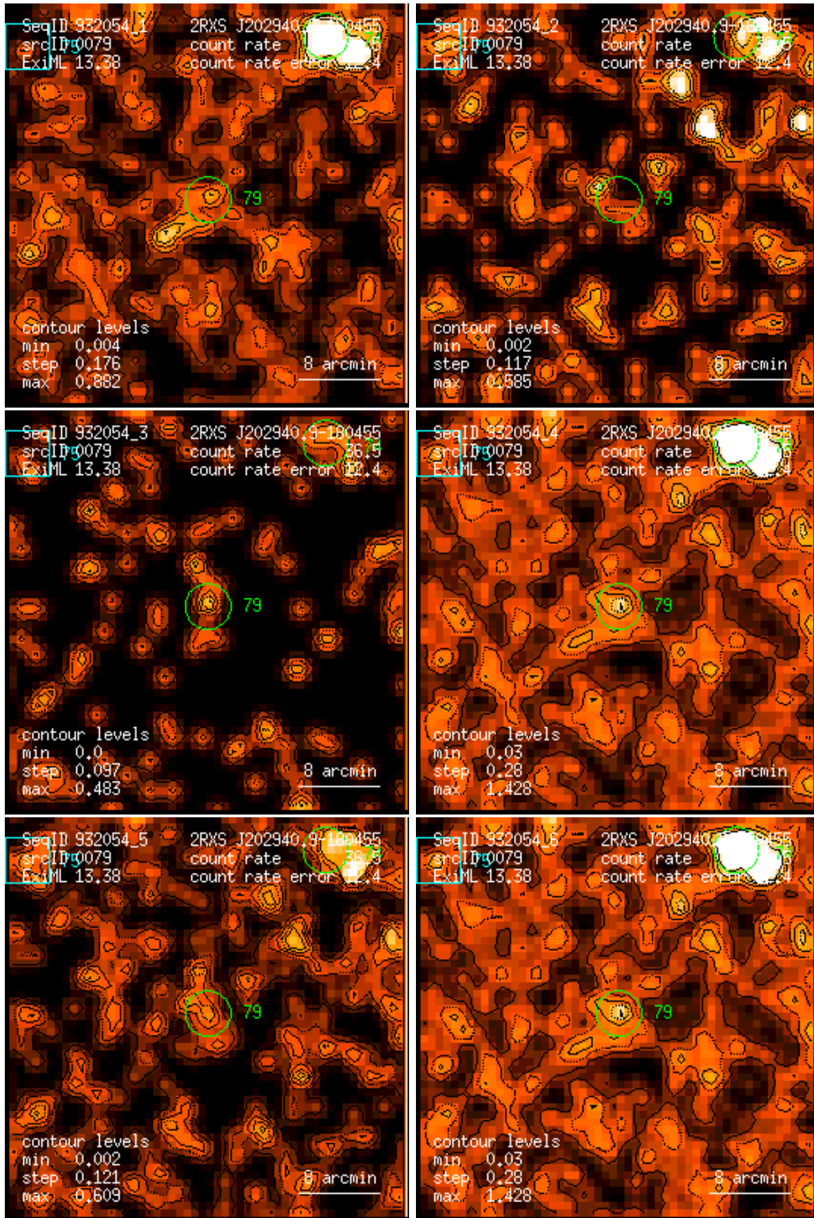
Figure 79: RASS 932054: detection 0079: band rate images, Gaussian filter: (1) PSPC channels 11 – 41, (2) 52 – 90, (3) 91 – 201, (4) 11 – 235, (5) 52 – 201, (6) 11 – 201. Broad band rates in counts/ks. Band rate contour levels in counts/ks/arcmin 2 .
