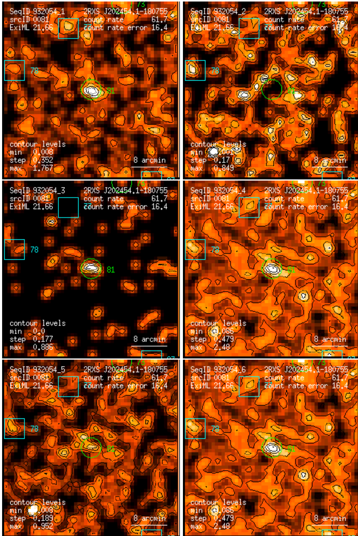
Figure 81: RASS 932054: detection 0081: band rate images, Gaussian filter: (1) PSPC channels 11 – 41, (2) 52 – 90, (3) 91 – 201, (4) 11 – 235, (5) 52 – 201, (6) 11 – 201. Broad band rates in counts/ks. Band rate contour levels in counts/ks/arcmin 2 .
