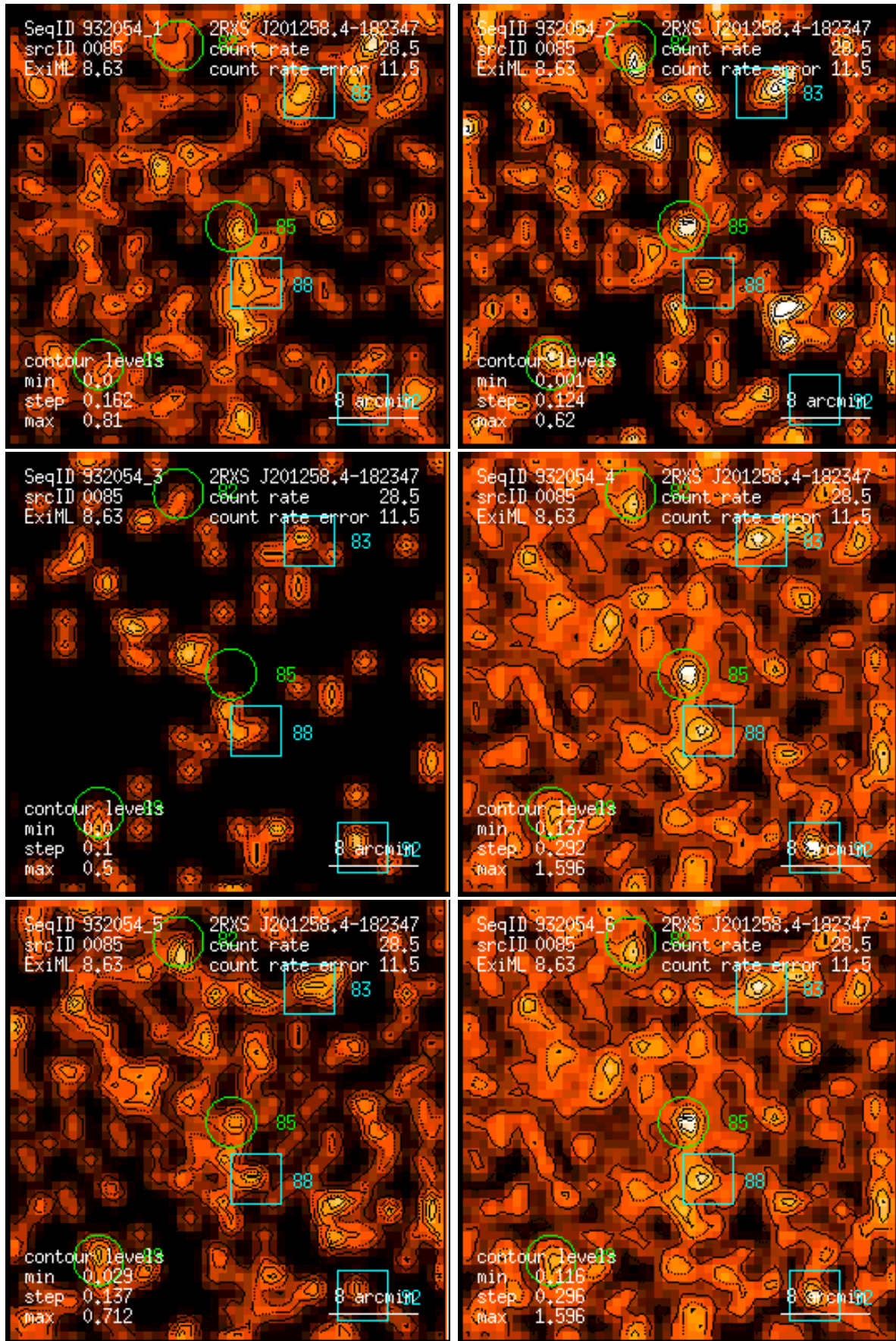
Figure 85: RASS 932054: detection 0085: band rate images, Gaussian filter: (1) PSPC channels 11 – 41, (2) 52 – 90, (3) 91 – 201, (4) 11 – 235, (5) 52 – 201, (6) 11 – 201. Broad band rates in counts/ks. Band rate contour levels in counts/ks/arcmin 2 .
