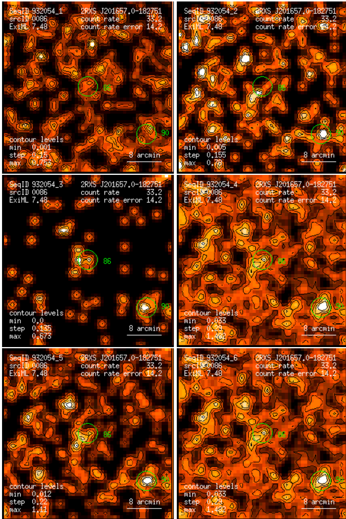
Figure 86: RASS 932054: detection 0086: band rate images, Gaussian filter: (1) PSPC channels 11 – 41, (2) 52 – 90, (3) 91 – 201, (4) 11 – 235, (5) 52 – 201, (6) 11 – 201. Broad band rates in counts/ks. Band rate contour levels in counts/ks/arcmin 2 .
