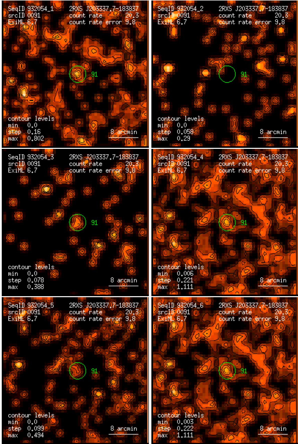
Figure 91: RASS 932054: detection 0091: band rate images, Gaussian filter: (1) PSPC channels 11 – 41, (2) 52 – 90, (3) 91 – 201, (4) 11 – 235, (5) 52 – 201, (6) 11 – 201. Broad band rates in counts/ks. Band rate contour levels in counts/ks/arcmin 2 .
