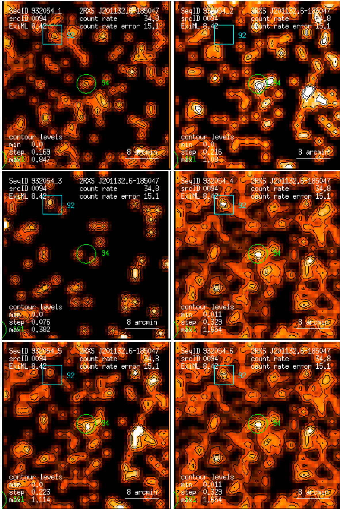
Figure 94: RASS 932054: detection 0094: band rate images, Gaussian filter: (1) PSPC channels 11 – 41, (2) 52 – 90, (3) 91 – 201, (4) 11 – 235, (5) 52 – 201, (6) 11 – 201. Broad band rates in counts/ks. Band rate contour levels in counts/ks/arcmin 2 .
