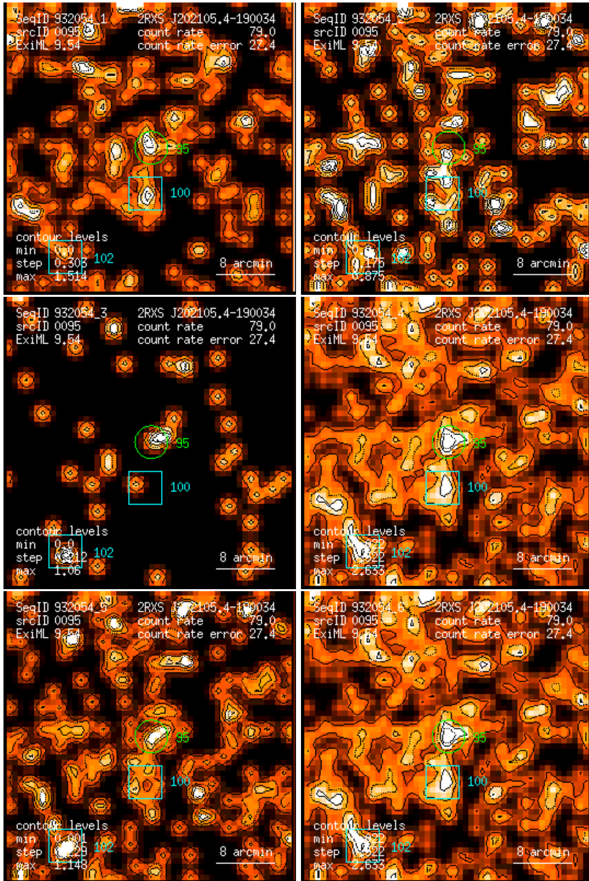
Figure 95: RASS 932054: detection 0095: band rate images, Gaussian filter: (1) PSPC channels 11 – 41, (2) 52 – 90, (3) 91 – 201, (4) 11 – 235, (5) 52 – 201, (6) 11 – 201. Broad band rates in counts/ks. Band rate contour levels in counts/ks/arcmin 2 .
