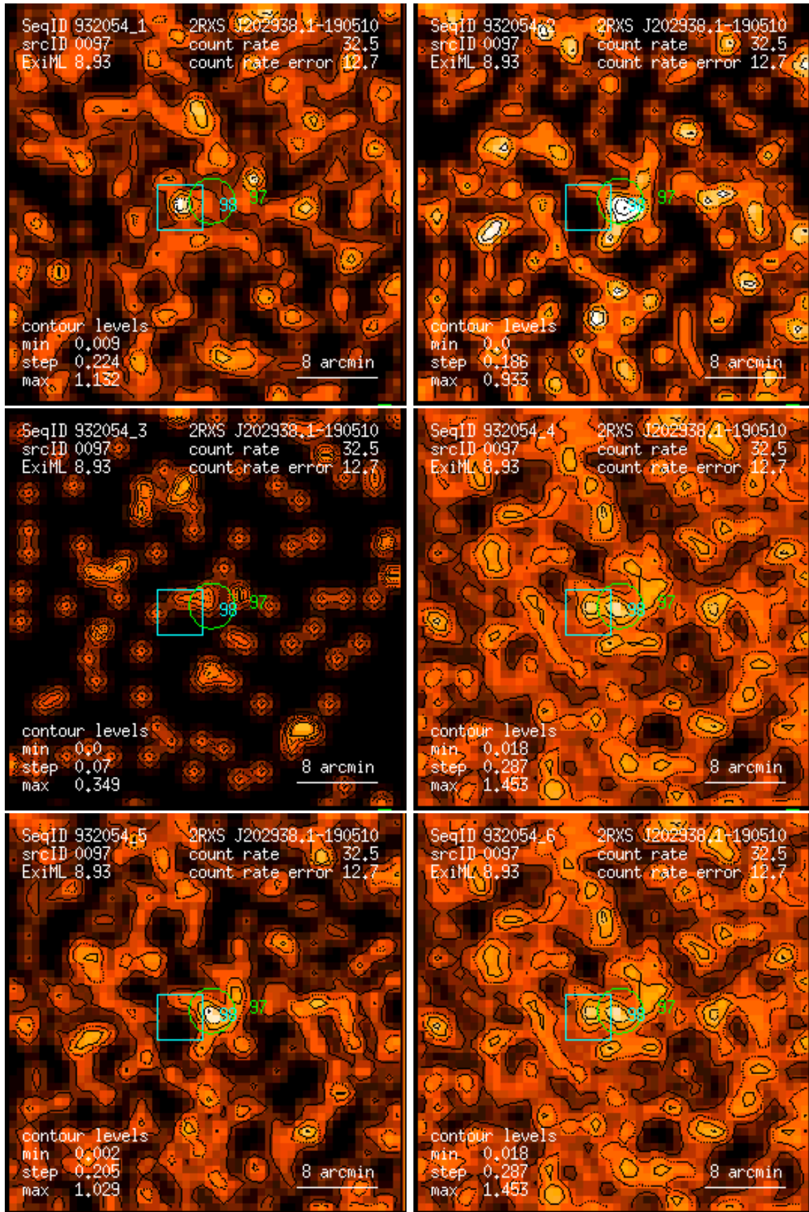
Figure 97: RASS 932054: detection 0097: band rate images, Gaussian filter: (1) PSPC channels 11 – 41, (2) 52 – 90, (3) 91 – 201, (4) 11 – 235, (5) 52 – 201, (6) 11 – 201. Broad band rates in counts/ks. Band rate contour levels in counts/ks/arcmin 2 .
