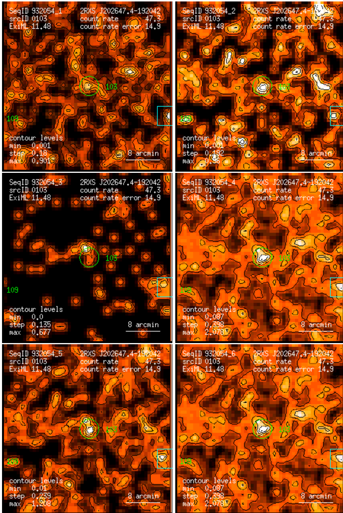
Figure 103: RASS 932054: detection 0103: band rate images, Gaussian filter: (1) PSPC channels 11 – 41, (2) 52 – 90, (3) 91 – 201, (4) 11 – 235, (5) 52 – 201, (6) 11 – 201. Broad band rates in counts/ks. Band rate contour levels in counts/ks/arcmin 2 .
