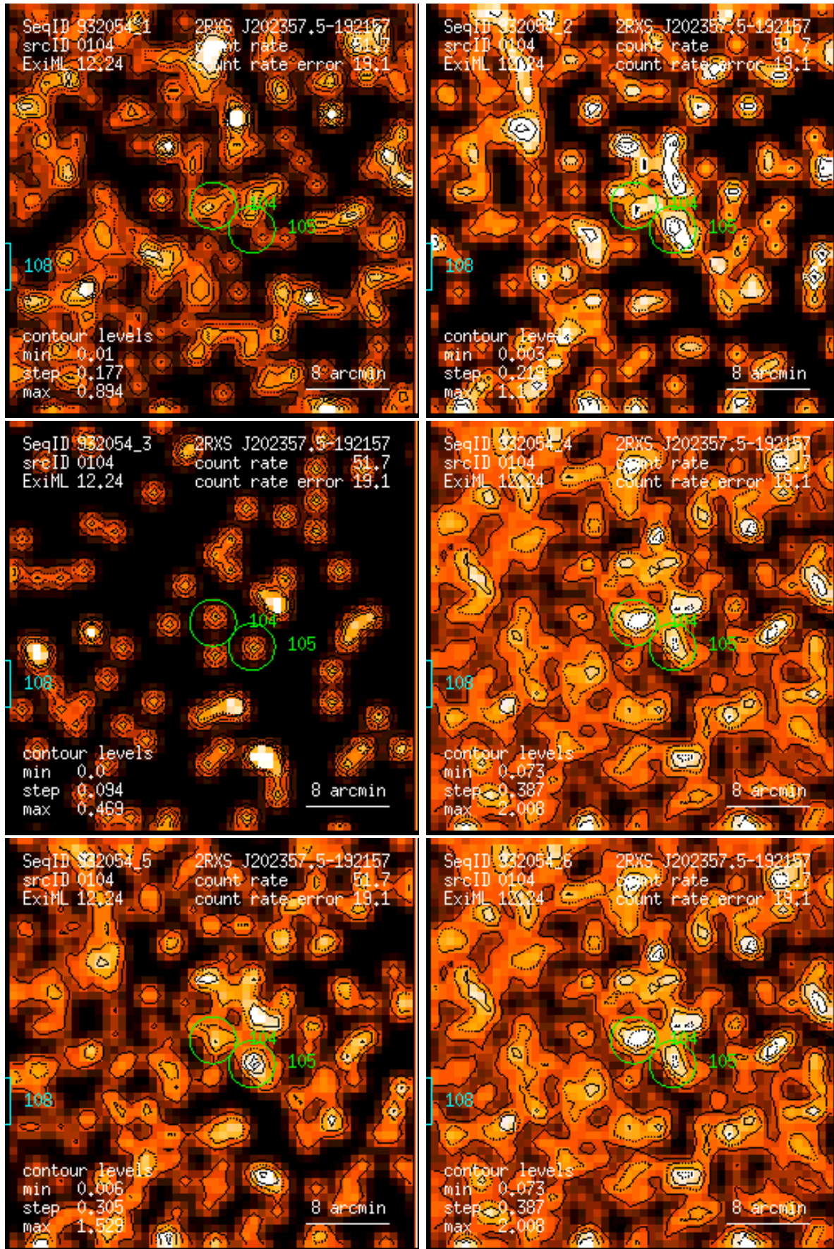
Figure 104: RASS 932054: detection 0104: band rate images, Gaussian filter: (1) PSPC channels 11 – 41, (2) 52 – 90, (3) 91 – 201, (4) 11 – 235, (5) 52 – 201, (6) 11 – 201. Broad band rates in counts/ks. Band rate contour levels in counts/ks/arcmin 2 .
