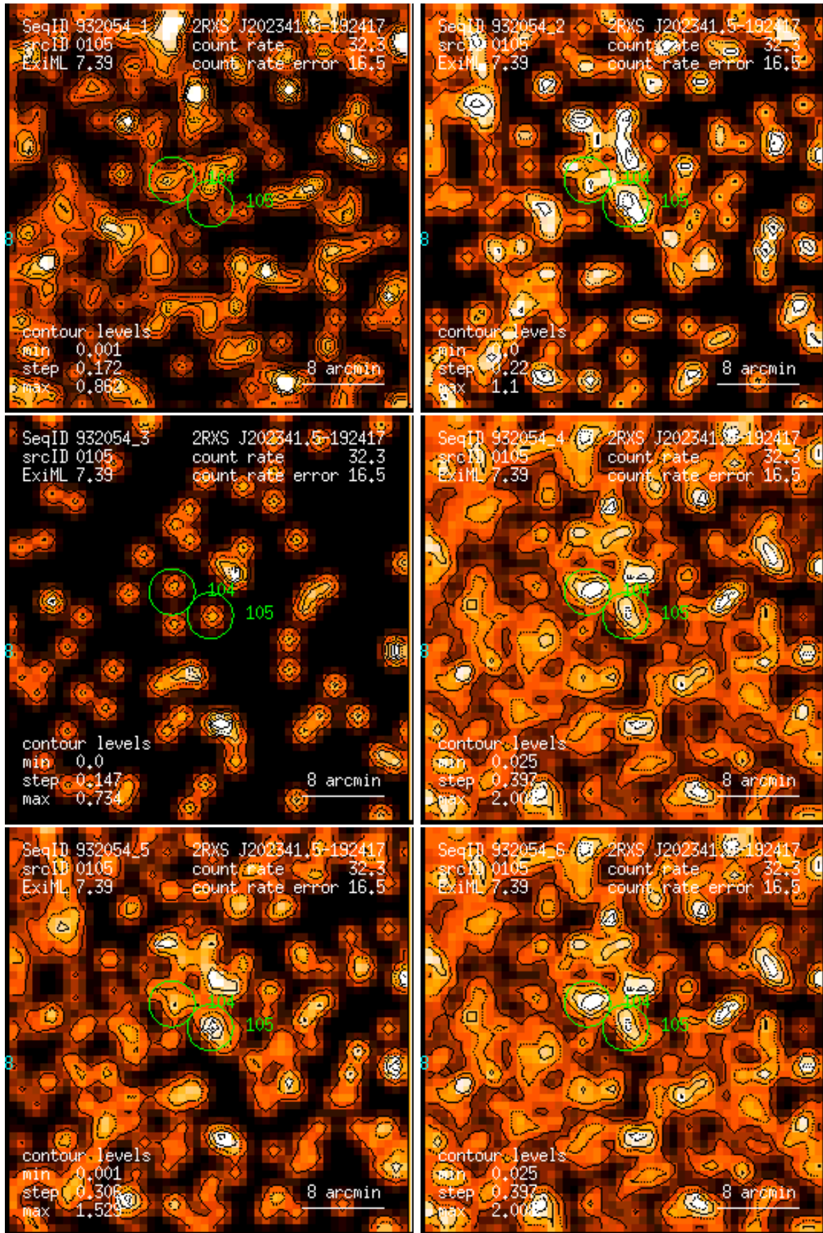
Figure 105: RASS 932054: detection 0105: band rate images, Gaussian filter: (1) PSPC channels 11 – 41, (2) 52 – 90, (3) 91 – 201, (4) 11 – 235, (5) 52 – 201, (6) 11 – 201. Broad band rates in counts/ks. Band rate contour levels in counts/ks/arcmin 2 .
