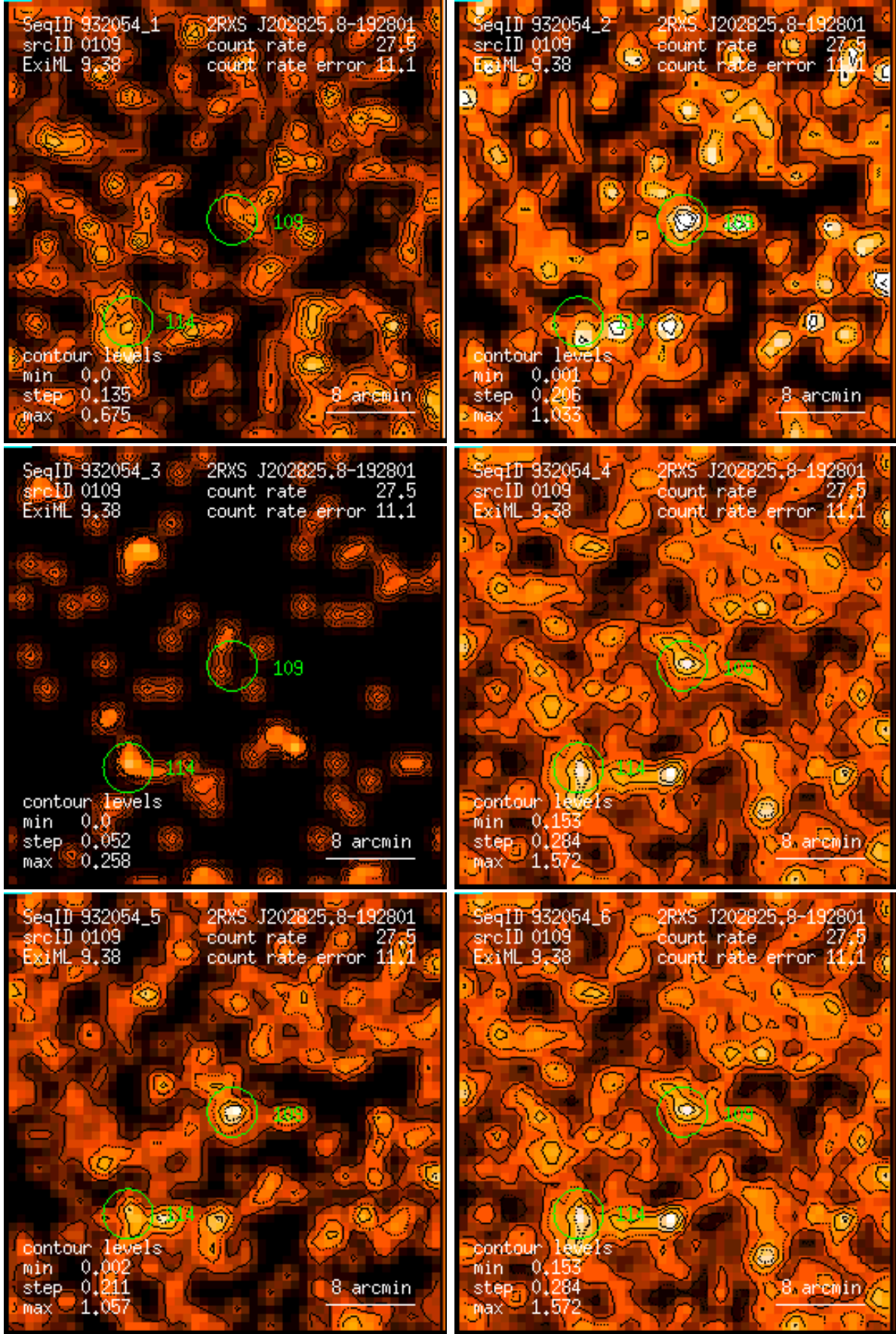
Figure 109: RASS 932054: detection 0109: band rate images, Gaussian filter: (1) PSPC channels 11 – 41, (2) 52 – 90, (3) 91 – 201, (4) 11 – 235, (5) 52 – 201, (6) 11 – 201. Broad band rates in counts/ks. Band rate contour levels in counts/ks/arcmin 2 .
