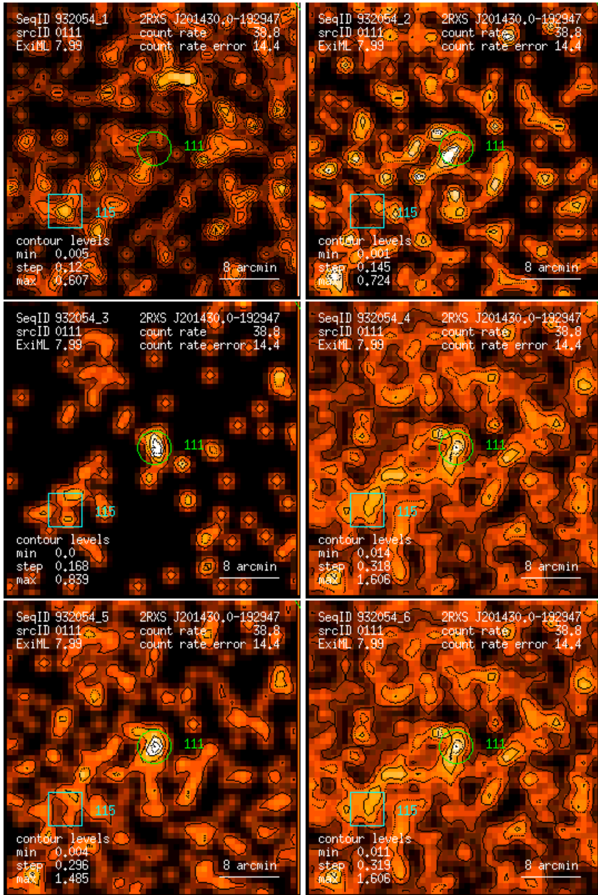
Figure 111: RASS 932054: detection 0111: band rate images, Gaussian filter: (1) PSPC channels 11 – 41, (2) 52 – 90, (3) 91 – 201, (4) 11 – 235, (5) 52 – 201, (6) 11 – 201. Broad band rates in counts/ks. Band rate contour levels in counts/ks/arcmin 2 .
