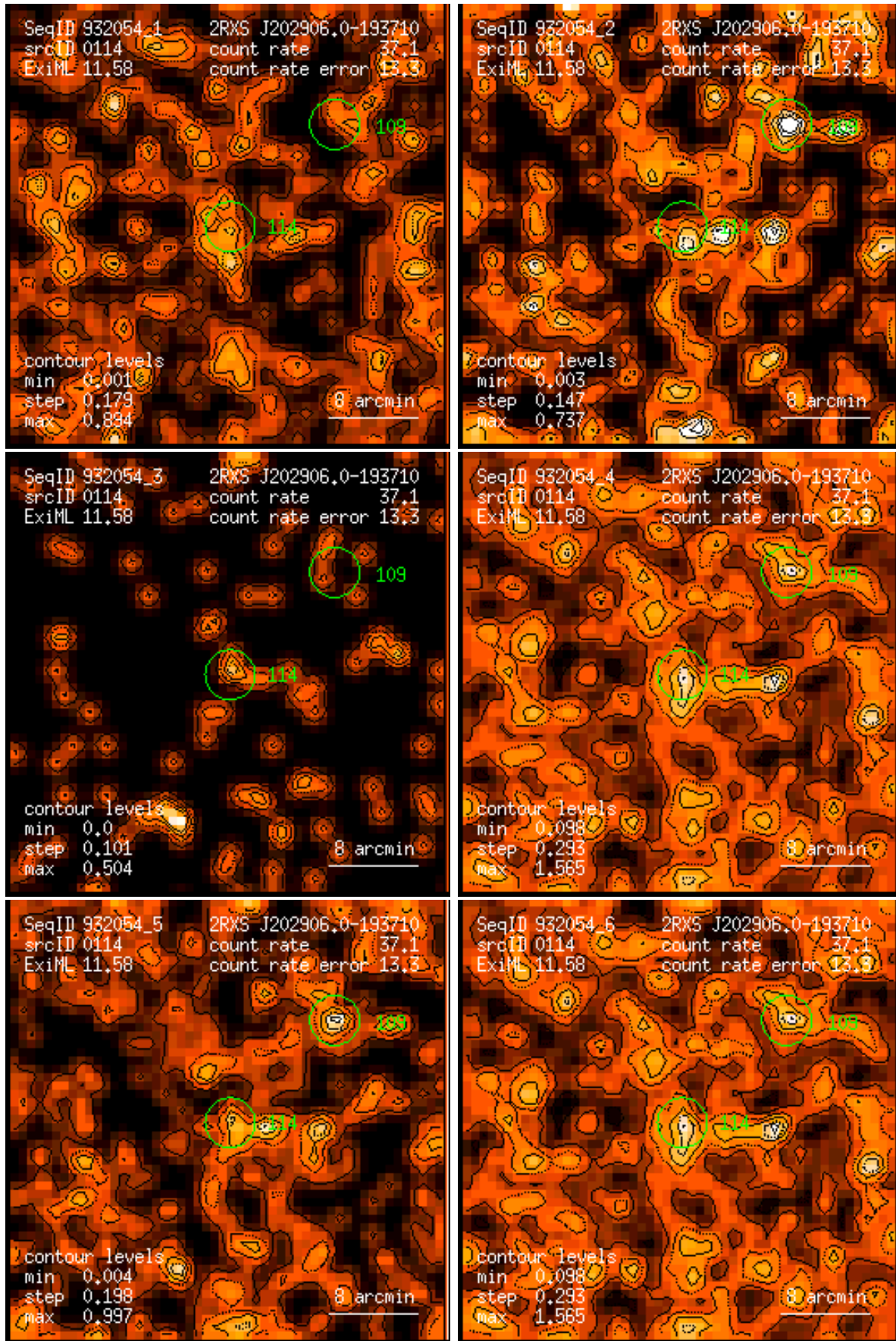
Figure 114: RASS 932054: detection 0114: band rate images, Gaussian filter: (1) PSPC channels 11 – 41, (2) 52 – 90, (3) 91 – 201, (4) 11 – 235, (5) 52 – 201, (6) 11 – 201. Broad band rates in counts/ks. Band rate contour levels in counts/ks/arcmin 2 .
