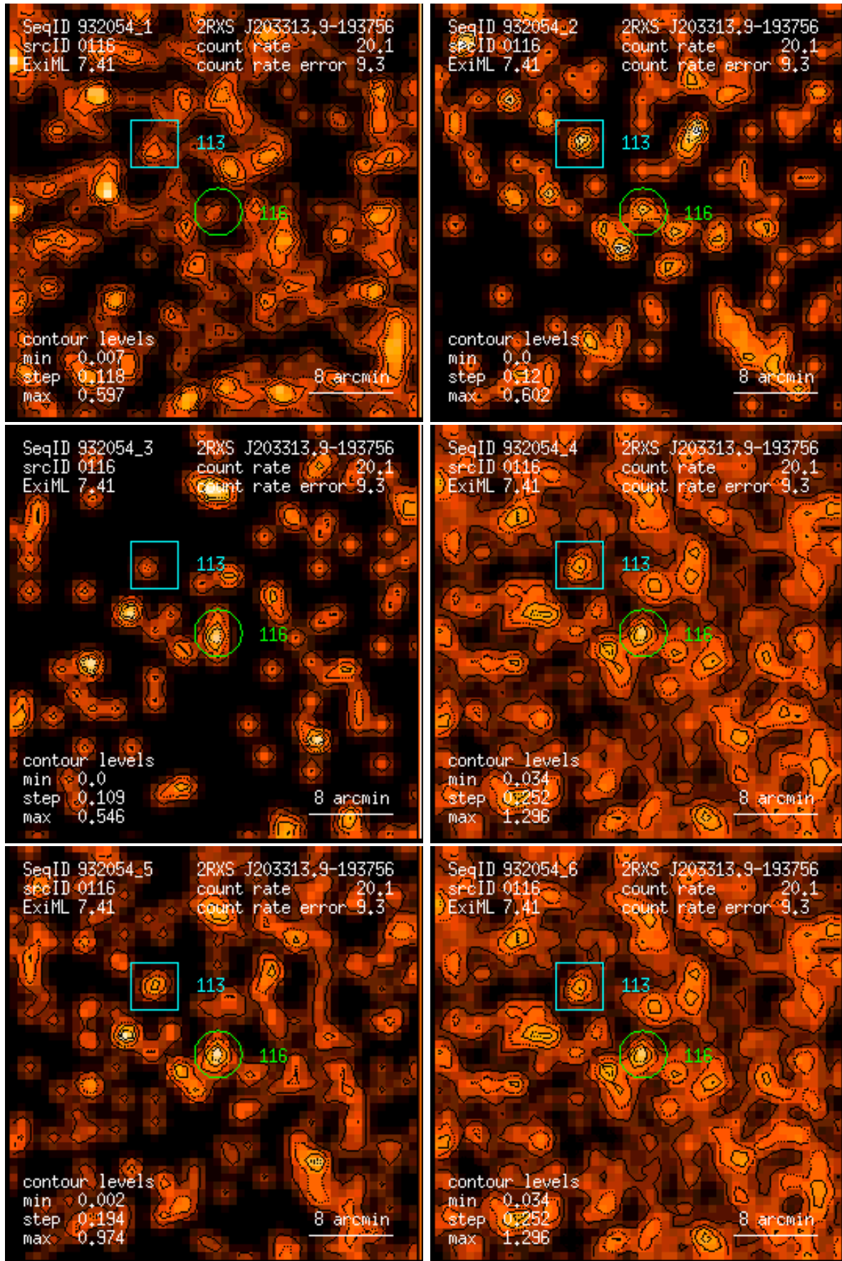
Figure 116: RASS 932054: detection 0116: band rate images, Gaussian filter: (1) PSPC channels 11 – 41, (2) 52 – 90, (3) 91 – 201, (4) 11 – 235, (5) 52 – 201, (6) 11 – 201. Broad band rates in counts/ks. Band rate contour levels in counts/ks/arcmin 2 .
