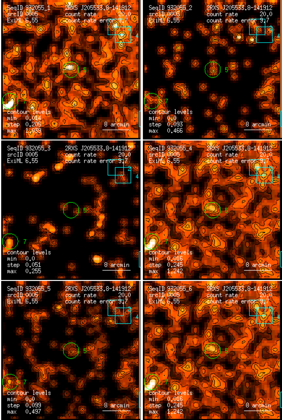
Figure 5: RASS 932055: detection 0005: band rate images, Gaussian filter: (1) PSPC channels 11 – 41, (2) 52 – 90, (3) 91 – 201, (4) 11 – 235, (5) 52 – 201, (6) 11 – 201. Broad band rates in counts/ks. Band rate contour levels in counts/ks/arcmin 2 .
