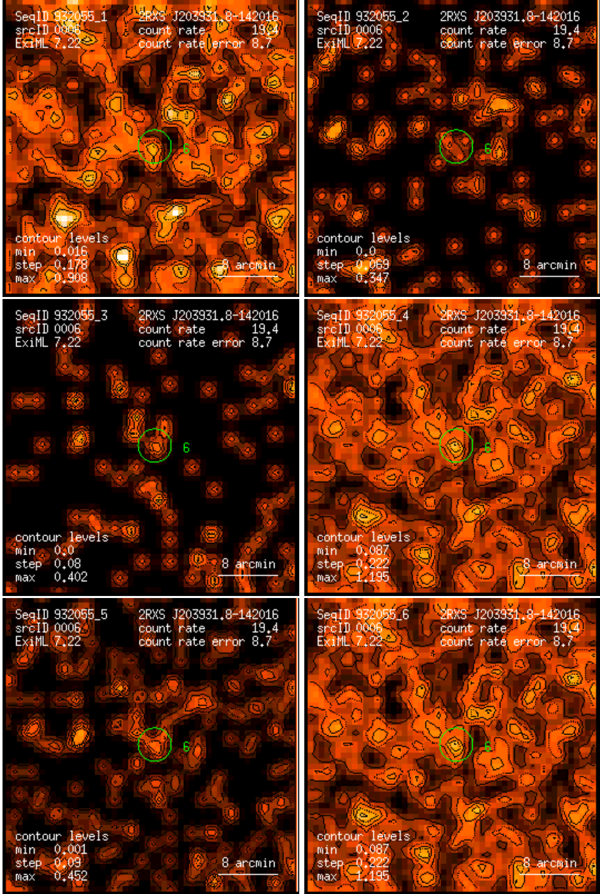
Figure 6: RASS 932055: detection 0006: band rate images, Gaussian filter: (1) PSPC channels 11 – 41, (2) 52 – 90, (3) 91 – 201, (4) 11 – 235, (5) 52 – 201, (6) 11 – 201. Broad band rates in counts/ks. Band rate contour levels in counts/ks/arcmin 2 .
