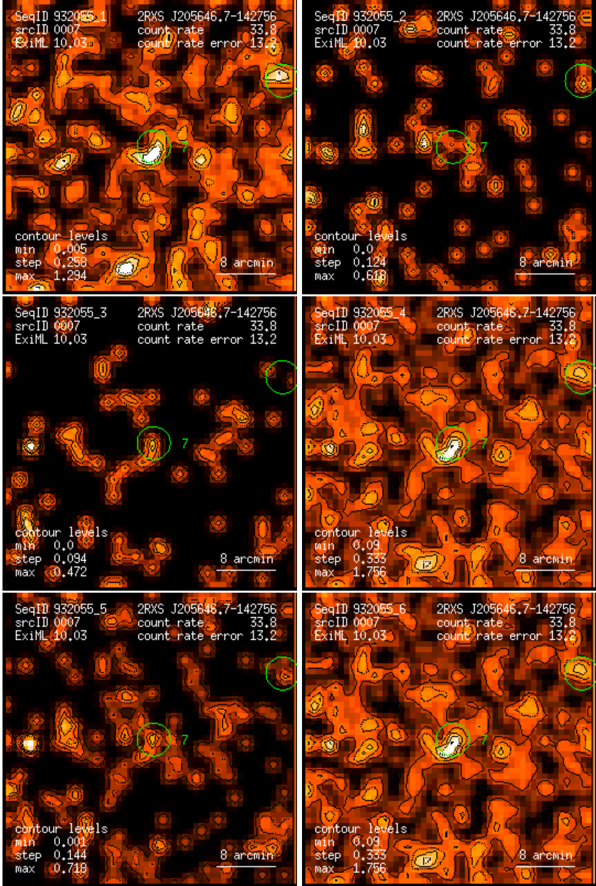
Figure 7: RASS 932055: detection 0007: band rate images, Gaussian filter: (1) PSPC channels 11 – 41, (2) 52 – 90, (3) 91 – 201, (4) 11 – 235, (5) 52 – 201, (6) 11 – 201. Broad band rates in counts/ks. Band rate contour levels in counts/ks/arcmin 2 .
