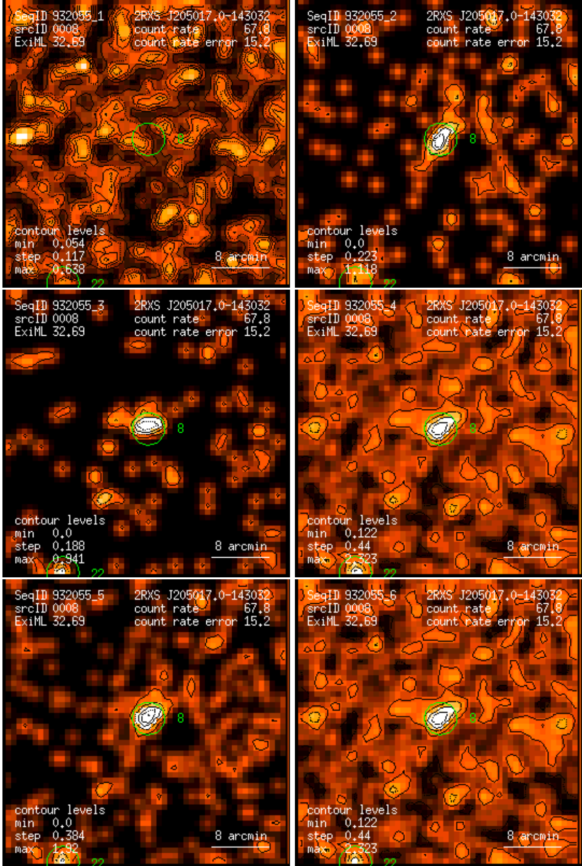
Figure 8: RASS 932055: detection 0008: band rate images, Gaussian filter: (1) PSPC channels 11 – 41, (2) 52 – 90, (3) 91 – 201, (4) 11 – 235, (5) 52 – 201, (6) 11 – 201. Broad band rates in counts/ks. Band rate contour levels in counts/ks/arcmin 2 .
