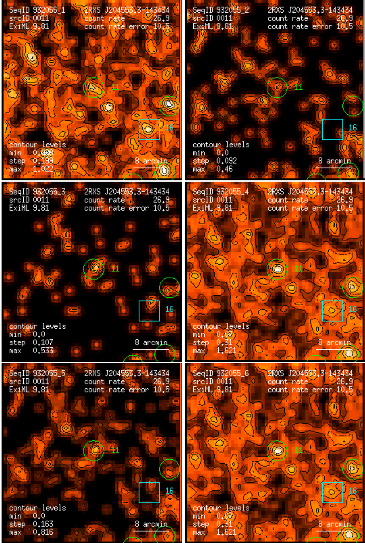
Figure 11: RASS 932055: detection 0011: band rate images, Gaussian filter: (1) PSPC channels 11 – 41, (2) 52 – 90, (3) 91 – 201, (4) 11 – 235, (5) 52 – 201, (6) 11 – 201. Broad band rates in counts/ks. Band rate contour levels in counts/ks/arcmin 2 .
