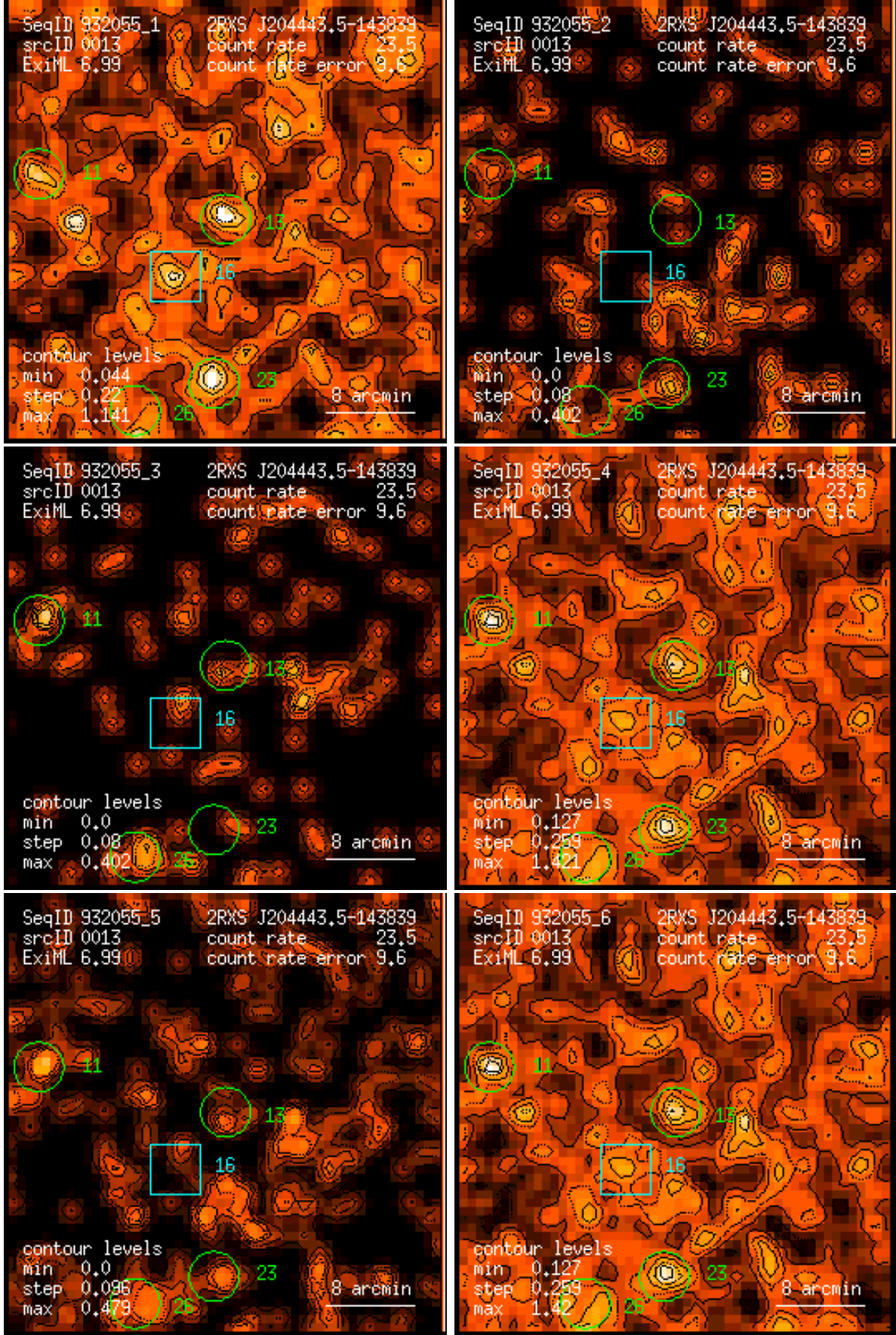
Figure 13: RASS 932055: detection 0013: band rate images, Gaussian filter: (1) PSPC channels 11 – 41, (2) 52 – 90, (3) 91 – 201, (4) 11 – 235, (5) 52 – 201, (6) 11 – 201. Broad band rates in counts/ks. Band rate contour levels in counts/ks/arcmin 2 .
