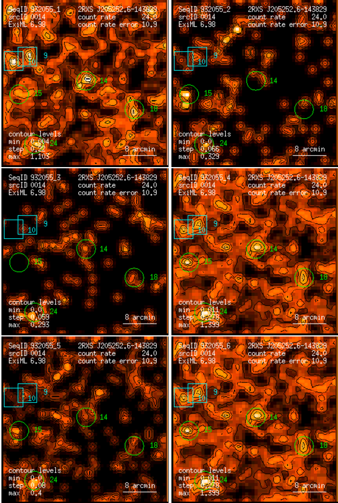
Figure 14: RASS 932055: detection 0014: band rate images, Gaussian filter: (1) PSPC channels 11 – 41, (2) 52 – 90, (3) 91 – 201, (4) 11 – 235, (5) 52 – 201, (6) 11 – 201. Broad band rates in counts/ks. Band rate contour levels in counts/ks/arcmin 2 .
